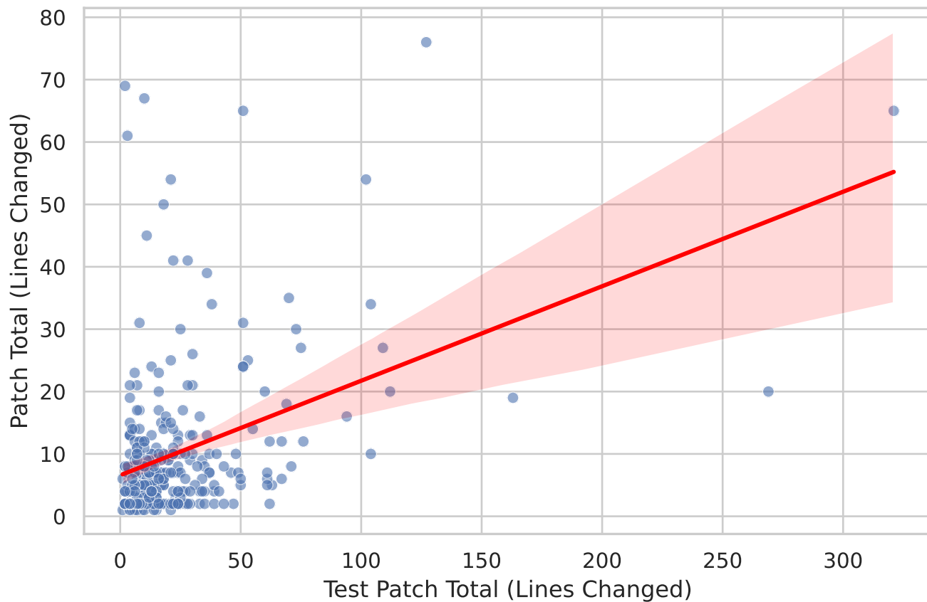
Patch Total vs Test Patch Total
