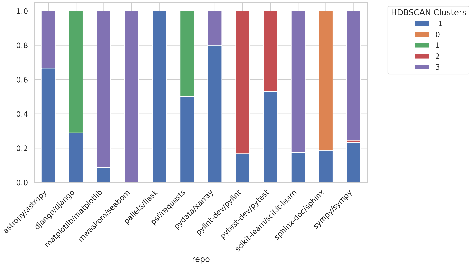
HDBSCAN clusters Distribution Over Repos
