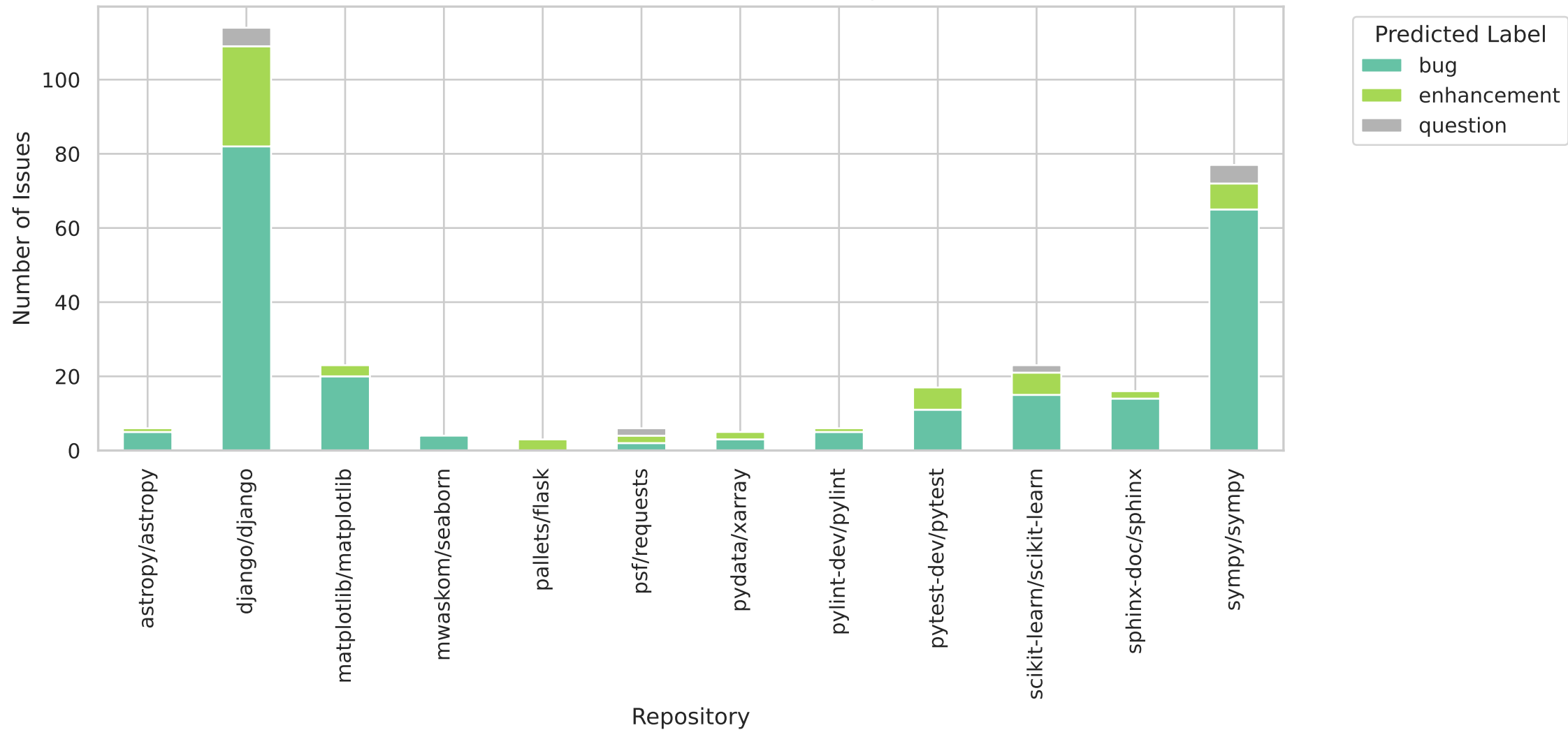
Distribution of Predicted Labels Across Repositories
