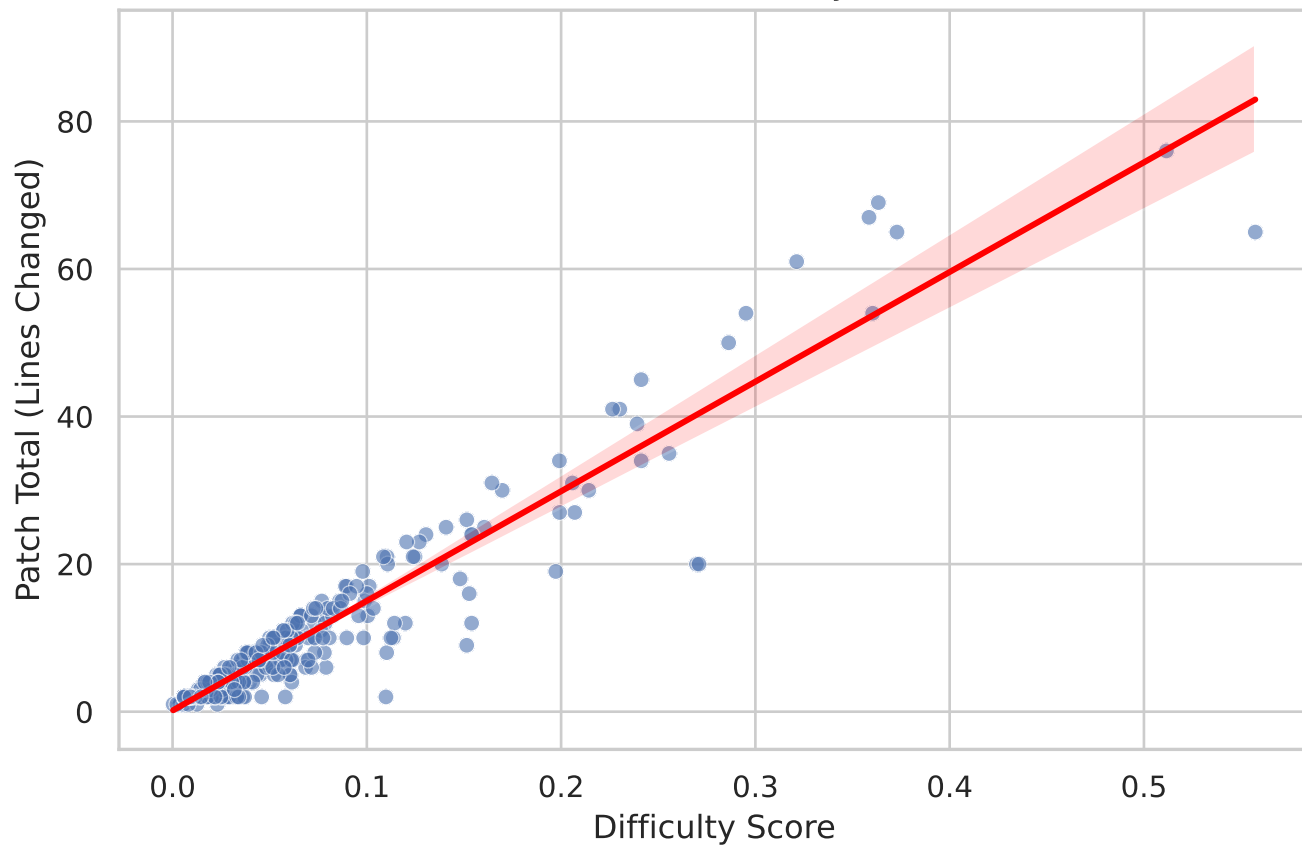
Patch Total vs Difficulty Score
