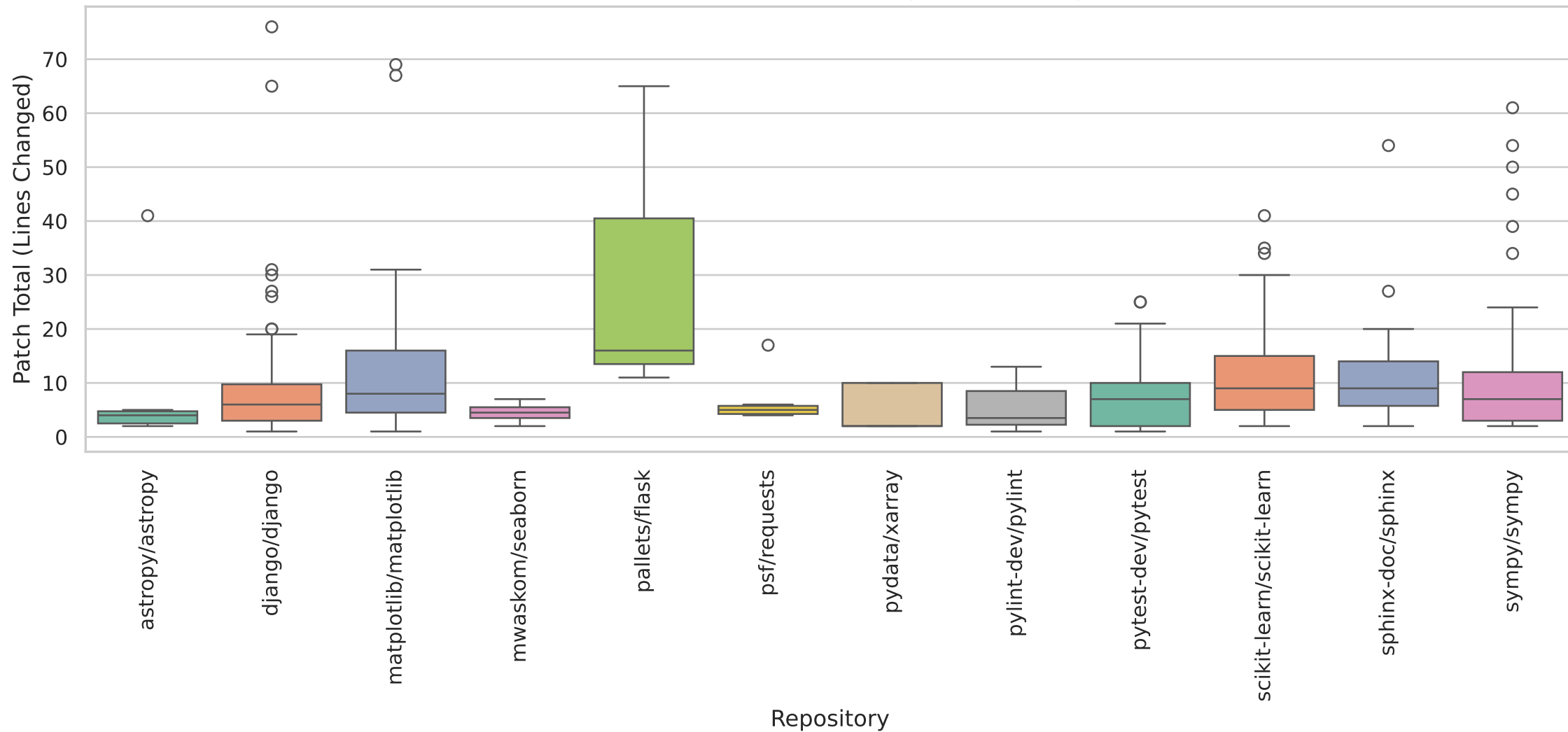
Patch Total Distribution Across Repositories (Boxplot)
