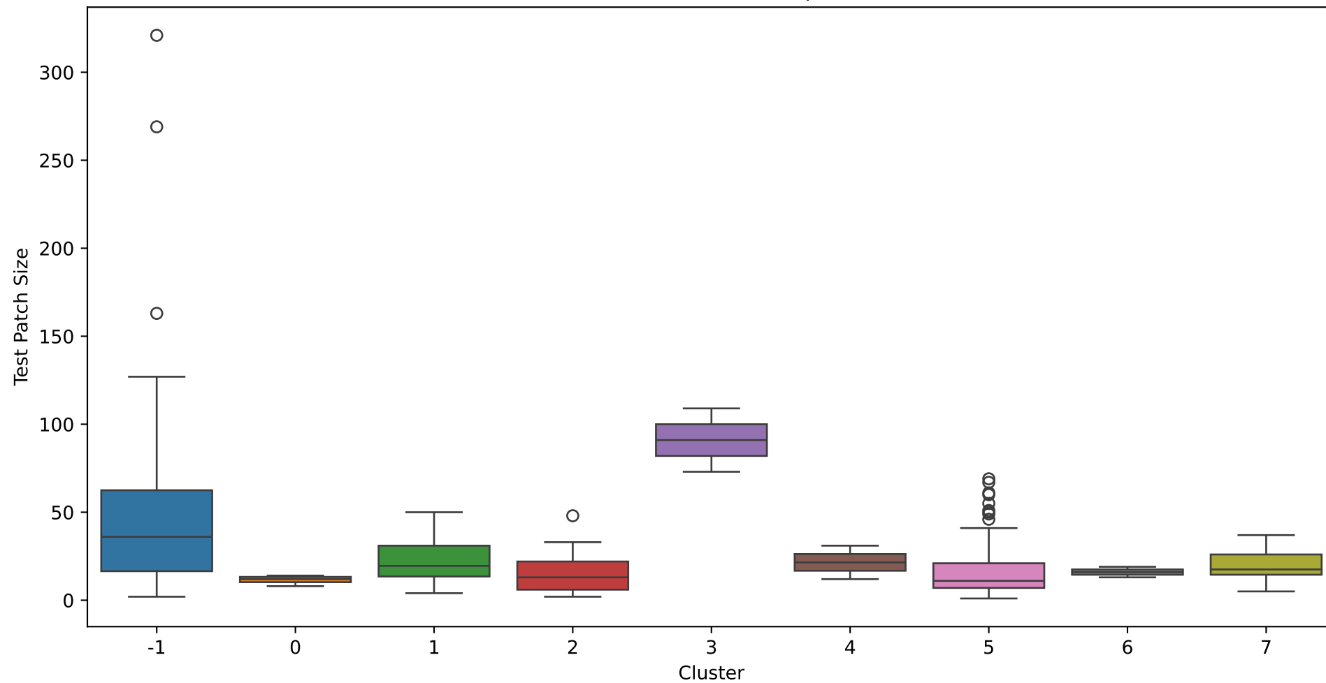
Test Patch Size Distribution per Cluster
