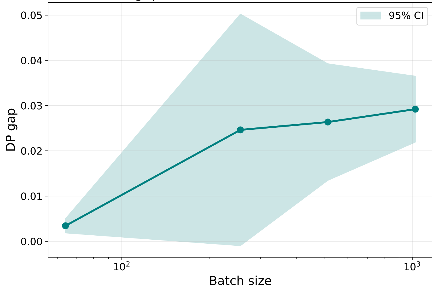
DP gap vs batch size UCI Credit Card
