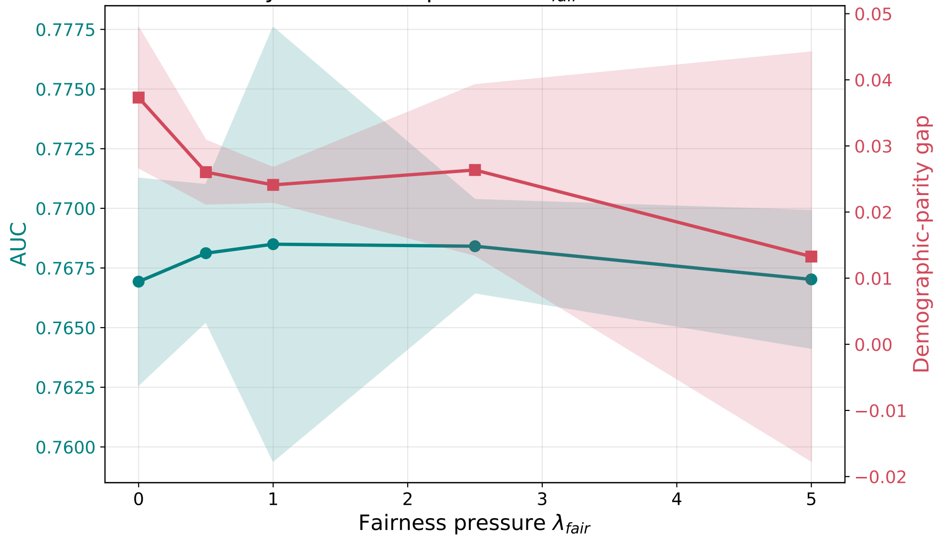
Accuracy-fairness response to \lambda_{fair} UCI Credit Card
