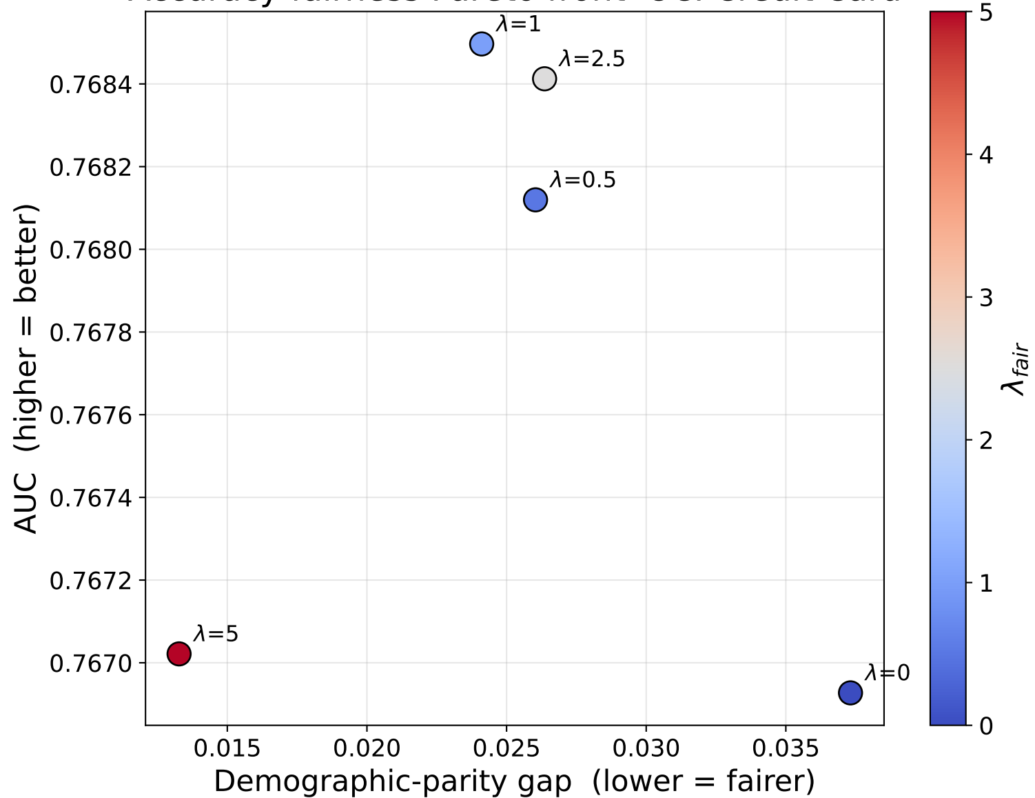
Accuracy-fairness Pareto front UCI Credit Card
