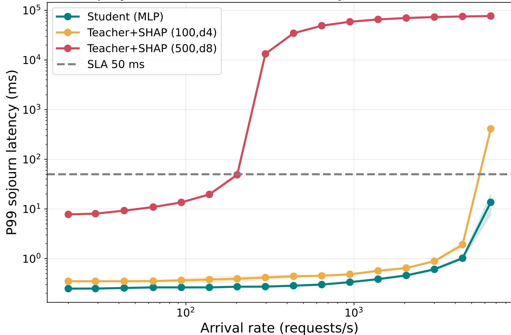
Deployment under load: tail latency (creditcard, c=1)
