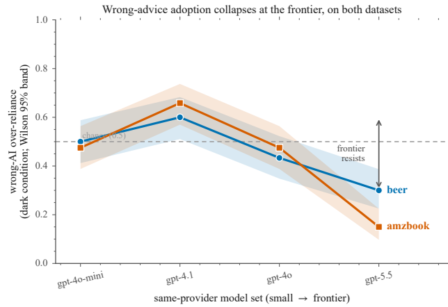
Figure 1: Axis-2 wrong-advice adoption on the guaranteed-wrong interface across the same-provider model set (gpt-4o-mini → gpt-4.1 → gpt-4o → gpt-5.5), both datasets (Wilson 95% CIs; dashed line = 0.5). Adoption is non-monotonic across backends; gpt-5.5 has the lowest adoption on both datasets. The matched framing contrast (Section 5.3) provides a non-arbitrary baseline for this low level.
