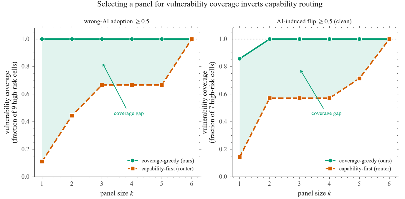
Figure 7: Vulnerability coverage as submodular set-cover. Each curve is the fraction of high-severity failure cells (dataset×persona reaching the risk threshold) a panel reproduces as it grows. Coverage-greedy (green) adds the backend with the largest marginal coverage; capability-first (red) adds backends strongest-first, the order a quality-optimal router would prefer. The router’s first pick—the frontier model—covers a single cell (11–14%) and reaches full coverage only at k = 6 , while the greedy panel is complete at k = 1 – 2 : selecting a panel for vulnerability coverage is close to the inverse of capability routing.
