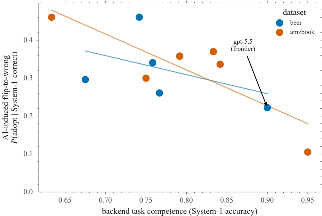
Capability vs AI-induced flip (directional, n = 6 )
