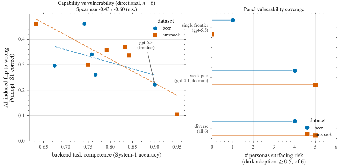
Fig. 7. Left: backend task competence (System-1 accuracy) vs. the AI-induced flip rate P(\text{adopt} | \text{System-1 correct}) , both datasets—a directional negative trend (Spearman -0.43 / -0.60 ; n.s. at n = 6 ). Right: vulnerability coverage (number of the six personas whose dark adoption reaches 0.5) for a single frontier backend, a weak pair, and the full panel. The single frontier backend surfaces the fewest at-risk profiles.
