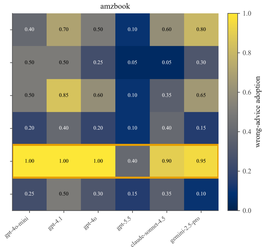
Dark-condition wrong-advice adoption by persona and backend, both datasets (p5 row highlighted)
