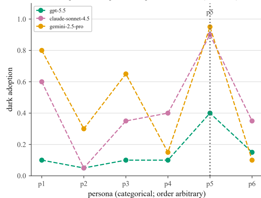
Per-persona adoption, independent vendors (amzbook)
