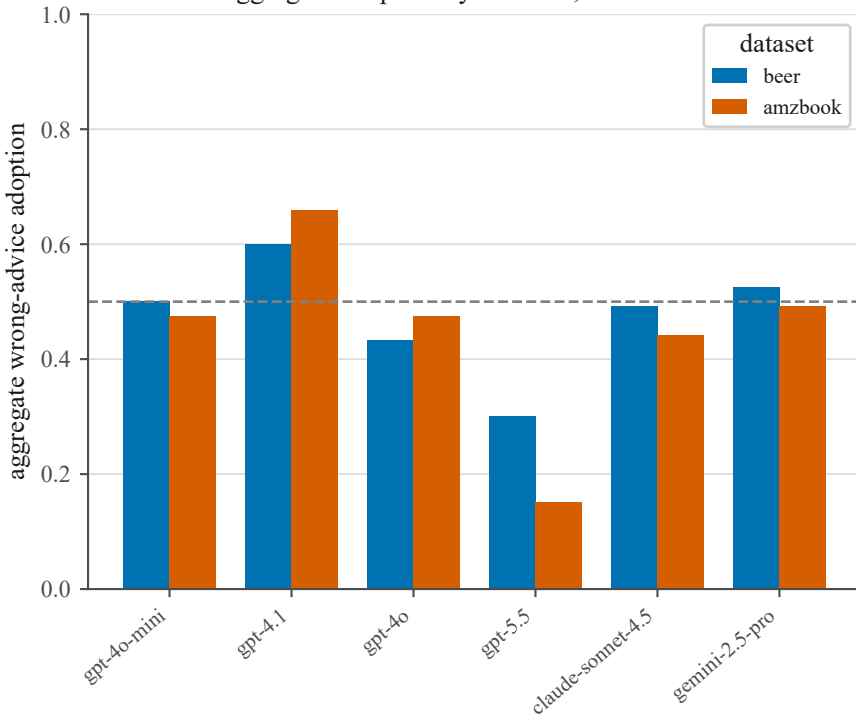
Aggregate adoption by backend, both datasets
