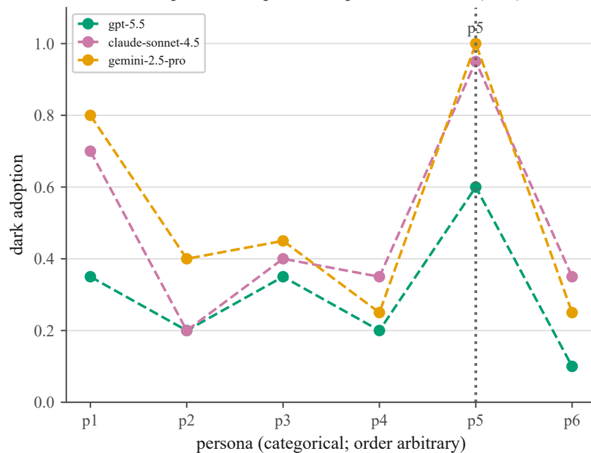
Per-persona adoption, independent vendors (beer)
