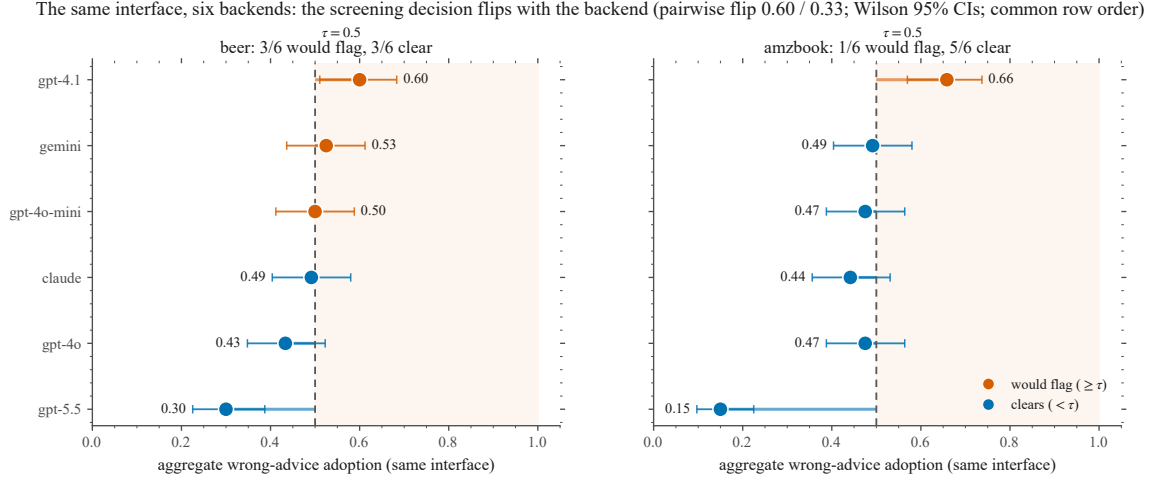
Fig. 2. The same guaranteed-wrong interface, scored by six backends, both datasets. Dots are aggregate wrong-advice adoption with Wilson 95% binomial CIs; the dashed line is a fixed decision threshold ( \tau = 0.5 ). Backends at or above threshold would flag the interface (red); the rest clear it (blue)—so the screening decision flips with the backend (pairwise flip rate 0.60 beer / 0.33 amzbook). Several mid-adoption backends have CIs that straddle \tau : the flip rate measures decision instability across backends, not a claim that each individual crossing is significant—the threshold-free companions (adoption range 0.15–0.66, Fleiss’ \kappa ) carry the same reading without fixing \tau .
