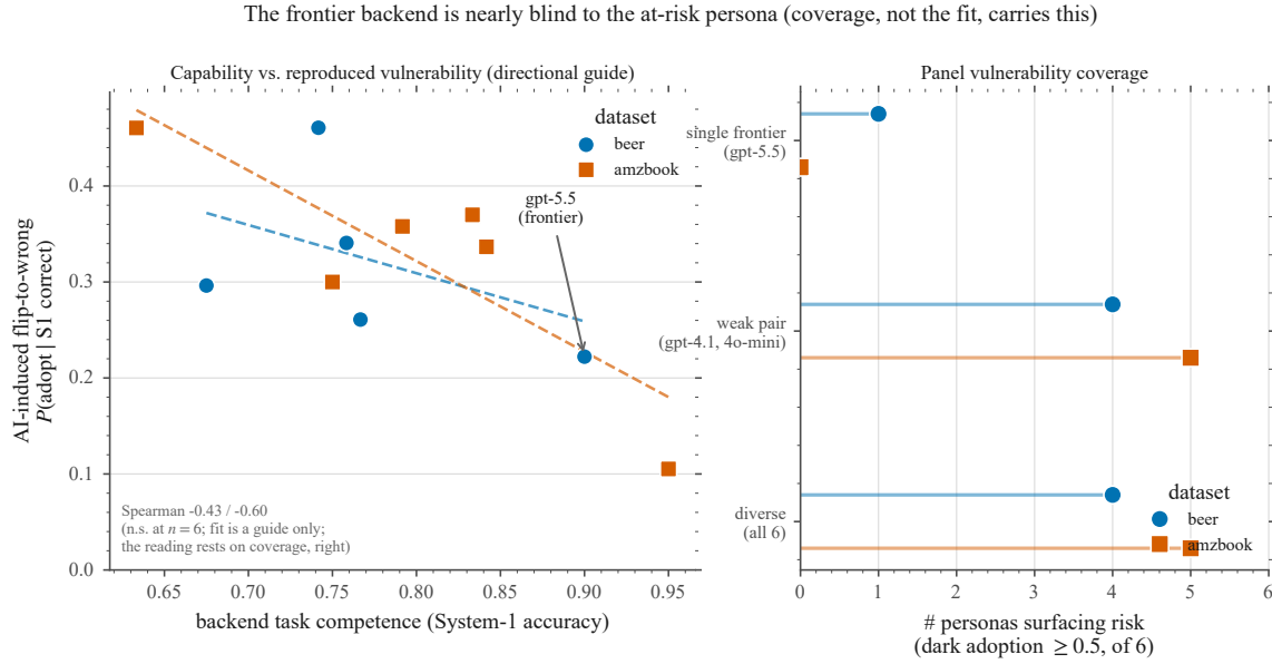
Fig. 7. The frontier backend under-represents the at-risk user. Left: backend task competence (System-1 accuracy) vs. the AI-induced flip rate P(\text{adopt} \mid \text{System-1 correct}) , both datasets—a directional negative trend (Spearman -0.43 / -0.60 ; n.s. at n = 6 , so the fit is a visual guide, not the load-bearing evidence). Right: vulnerability coverage (number of the six personas whose dark adoption reaches 0.5) for a single frontier backend, a weak pair, and the full panel—the model-free reading the argument rests on: the single frontier backend surfaces the fewest at-risk profiles.
