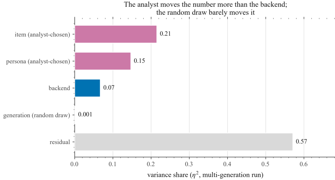
Fig. 3. What moves a synthetic-panel risk number. Variance shares ( \eta^2 ) from the preregistered multi-generation run (three backends \times two UI conditions \times six personas \times 20 items \times five generation seeds; 3,600 trials). The analyst-chosen item and persona dominate; the backend is a modest share; the random generation draw is essentially zero ( \eta^2 = 0.001 ). (This per-trial decomposition is not in tension with cross-backend aggregate instability, Section 5.3: a modest per-trial share still shifts the aggregate estimate enough to flip the decision.)
