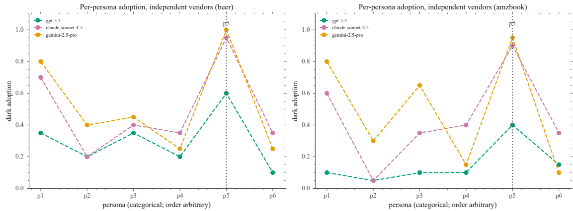
Fig. 6. Per-persona wrong-advice adoption profiles for the three independent-vendor backends, one panel per dataset. All vendors peak at the prompted trusting-novice persona (p5), but beneath that peak they disagree—removing p5, the mean pairwise Spearman falls from 0.87 to 0.77 on beer and from 0.50 to 0.09 on amzbook. Persona order is categorical (arbitrary). The shared p5 peak is a property of the persona prompt, not population discovery.
