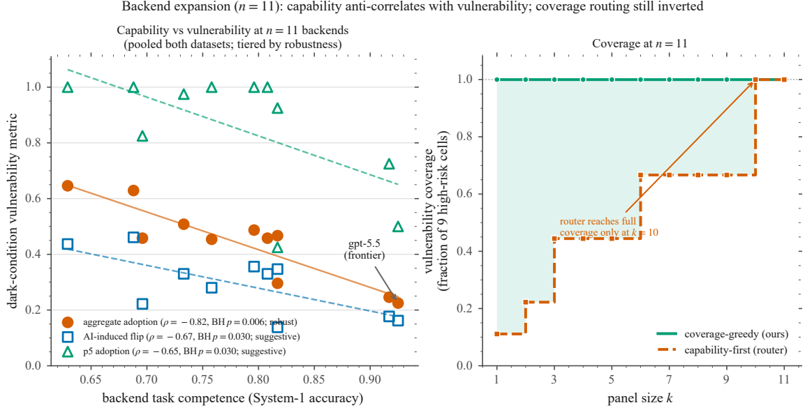
Fig. 8. Backend expansion to n = 11 (pooling both datasets). Left: backend task competence (System-1 accuracy) vs. three dark-condition vulnerability measures, tiered by robustness—aggregate adoption (filled, solid fit) is jackknife-robust and significant in each dataset; AI-induced flip and p5 adoption (open, dashed fit) are BH-significant only pooled and are amzbook-carried / single-backend fragile. Right: the n = 11 vulnerability-coverage curve—a capability-first (router) panel reaches full coverage of the high-risk cells only at k = 10 , while a coverage-greedy panel is complete almost immediately; a single frontier backend covers 1/9.
