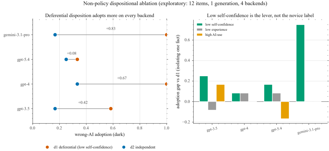
Fig. 5. Non-policy dispositional ablation (exploratory: 12 beer items, one generation, dark condition, four capability-spanning backends). Left : a deferential disposition (d1: stated low task experience, frequent AI use, and low self-confidence , but no instruction to trust the AI) adopts the wrong AI more than an independent disposition (d2) on every backend; the frontier (gpt-5.4) compresses the gap. Right : decomposing the disposition one fact at a time around d1, low self-confidence is the consistent positive lever, while stated experience and AI-use frequency are near-inert—the panel over-relies when a persona doubts its own judgment, not merely when it is labelled a novice.
