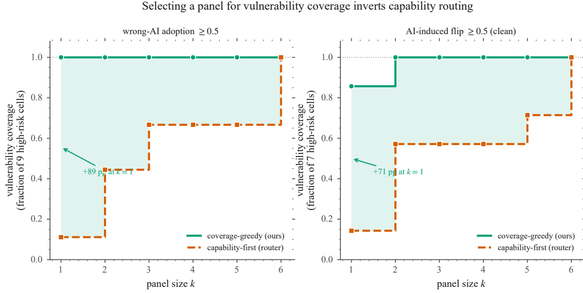
Fig. 7. Adding the strongest models first is the wrong strategy for surfacing interface risk. Each curve is the fraction of high-severity failure cells (dataset×persona reaching the risk threshold) a panel reproduces as it grows (formally, a submodular set-cover). Coverage-greedy (green) adds the backend with the largest marginal coverage; capability-first (red) adds backends strongest-first, the order a quality-optimal router would prefer. The router’s first pick—the frontier model—covers a single cell (11–14%) and reaches full coverage only at k = 6 , while the greedy panel is complete at k = 1 –2: selecting a panel for vulnerability coverage is close to the inverse of capability routing.
