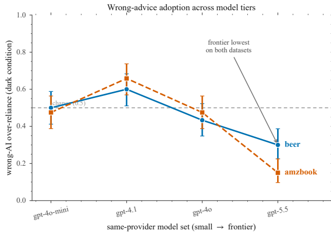
Figure 1: Axis-2 wrong-advice adoption on the guaranteed-wrong interface across the same-provider model set (gpt-4o-mini → gpt-4.1 → gpt-4o → gpt-5.5), both datasets. Error bars are Wilson 95% binomial confidence intervals (descriptive; conflict-conditioned inference uses the item-clustered models below), and lines connect discrete model conditions only as a visual guide; dashed line = 0.5. Adoption is non-monotonic across backends; gpt-5.5 has the lowest adoption on both datasets. The matched framing contrast (Section 5.3) provides a non-arbitrary baseline for this low level.
