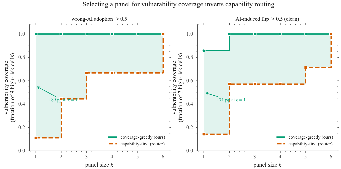
Figure 7: Vulnerability coverage as submodular set-cover. Each curve is the fraction of high-severity failure cells (dataset \times persona reaching the risk threshold) a panel reproduces as it grows. Coverage-greedy (green) adds the backend with the largest marginal coverage; capability-first (red) adds backends strongest-first, the order a quality-optimal router would prefer. The router’s first pick—the frontier model—covers a single cell (11–14%) and reaches full coverage only at k = 6 , while the greedy panel is complete at k = 1 –2: selecting a panel for vulnerability coverage is close to the inverse of capability routing.
