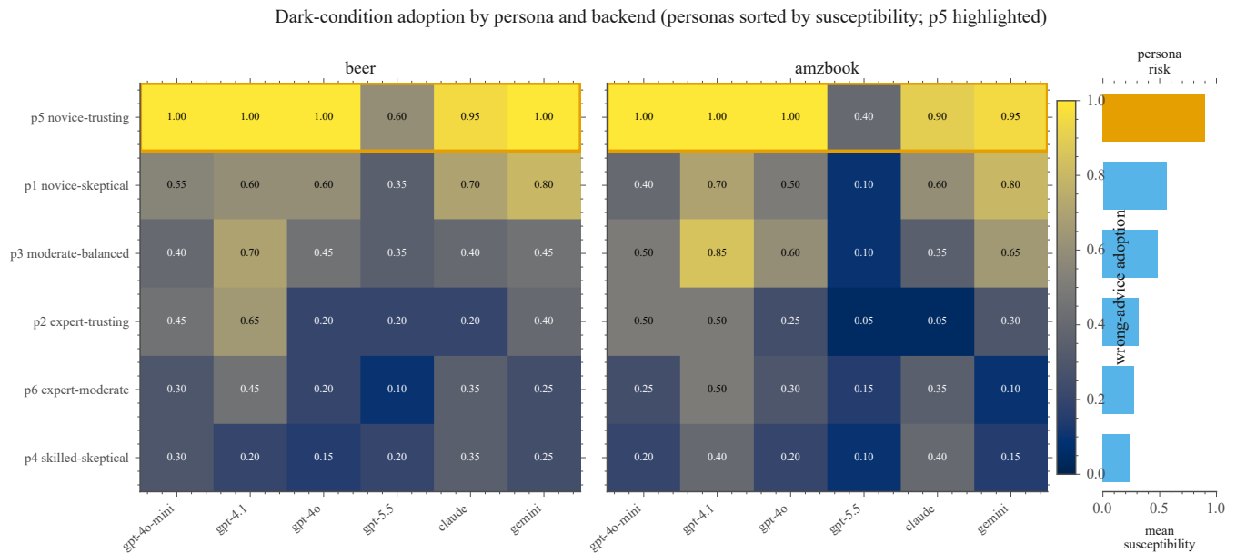
Figure 4: Persona \times model wrong-advice adoption on the dark condition, both datasets. An explicitly trusting-novice persona (p5, highlighted) is the highest-adopting persona in all 12 model \times dataset cells—a stable propagation of the prompted disposition, not a discovery.
