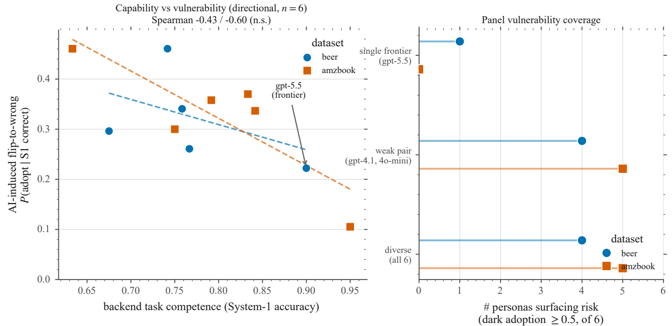
Figure 6: Left: backend task competence (System-1 accuracy) vs. the AI-induced flip rate P(\text{adopt} \mid \text{System-1 correct}) , both datasets—a directional negative trend (Spearman -0.43 / -0.60 ; n.s. at n=6 ). Right: vulnerability coverage (number of the six personas whose dark adoption reaches 0.5) for a single frontier backend, a weak pair, and the full panel. The single frontier backend surfaces the fewest at-risk profiles.
