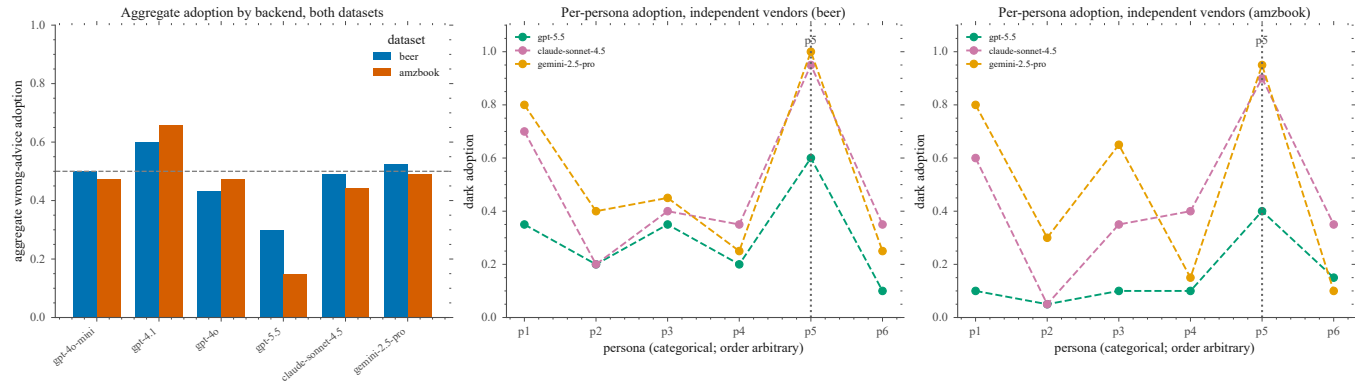
Figure 5: Left: aggregate wrong-advice adoption spans a wide range across backends on both datasets. Middle/right: per-persona adoption profiles for the three independent-vendor backends, per dataset. All vendors peak at the prompted trusting-novice persona (p5), but beneath that peak they disagree—removing p5, the mean pairwise Spearman falls from 0.87 to 0.77 on beer and from 0.50 to 0.09 on amzbook. Persona order is categorical (arbitrary). The shared p5 peak is a property of the persona prompt, not population discovery.
