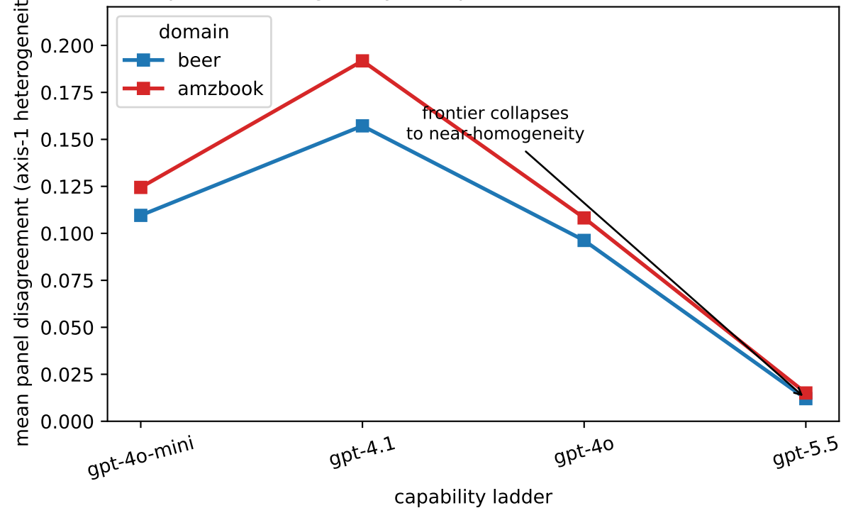
Axis-1 panel heterogeneity collapses at the frontier (both domains)
