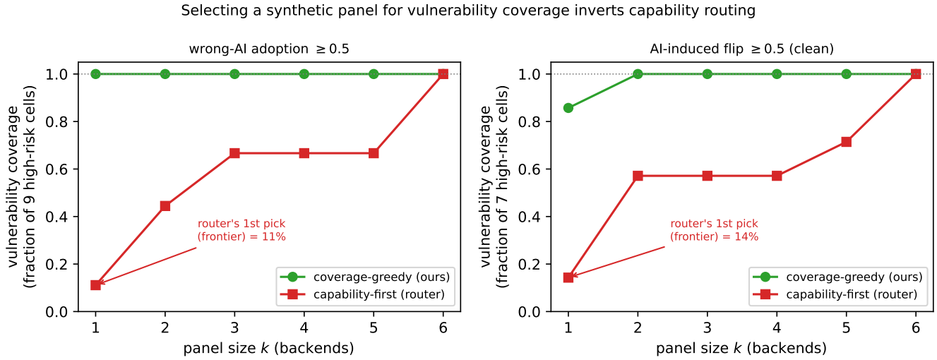
Figure 7: Vulnerability coverage as submodular set-cover. Each curve is the fraction of high-severity failure cells (dataset×persona reaching the risk threshold) a panel reproduces as it grows. Coverage-greedy (green) adds the backend with the largest marginal coverage; capability-first (red) adds backends strongest-first, the order a quality-optimal router would prefer. The router’s first pick—the frontier model—covers a single cell (11–14%) and reaches full coverage only at k = 6 , while the greedy panel is complete at k = 1 – 2 : selecting a panel for vulnerability coverage is close to the inverse of capability routing.
