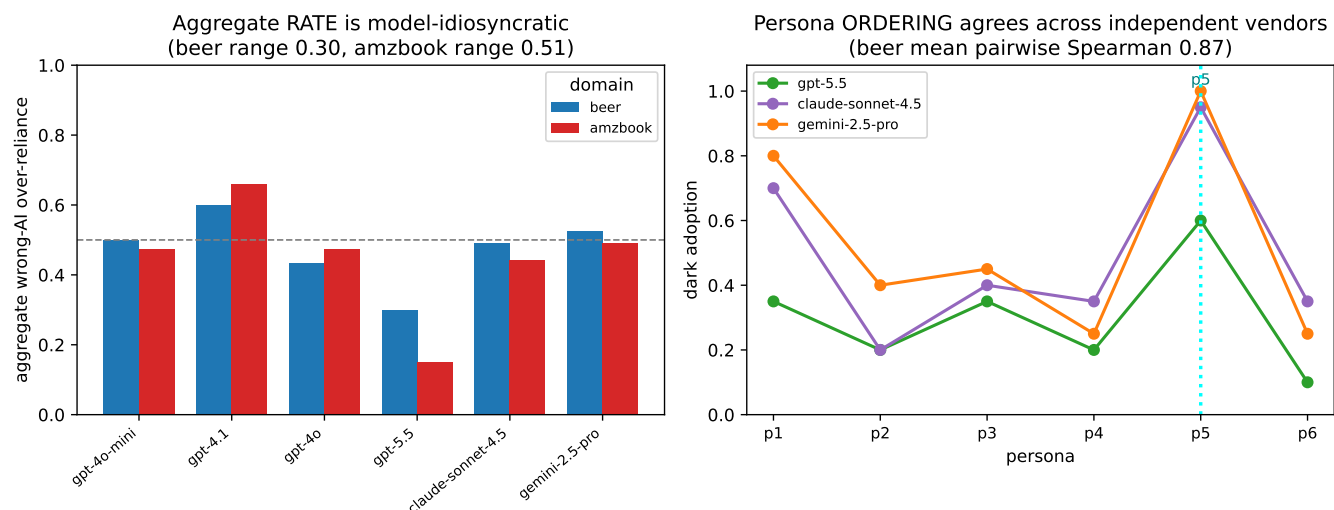
Figure 5: Left: aggregate wrong-advice adoption is model-idiosyncratic (large spread across models). Right: the per-persona adoption profile is consistent across independent vendors (gpt-5.5, claude, gemini), all peaking at the prompted trusting-novice persona (mean pairwise Spearman 0.87 on beer). This is a reliability property of persona-prompt propagation, not population discovery.
