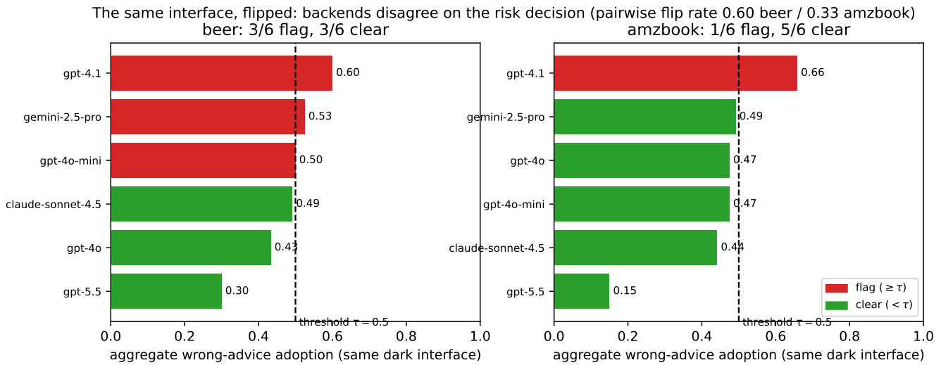
Figure 3: The same guaranteed-wrong interface, scored by six backends, both datasets. Bars are aggregate wrong-advice adoption; the dashed line is a fixed decision threshold ( \tau = 0.5 ). Red backends flag the interface, green backends clear it—so the screening decision flips with the backend (pairwise flip rate 0.60 beer / 0.33 amzbook).
