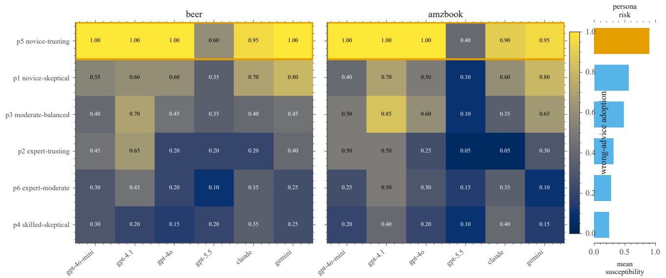
Figure 4: Persona \times model wrong-advice adoption on the dark condition, both datasets. An explicitly trusting-novice persona (p5, highlighted) is the highest-adopting persona in all 12 model \times dataset cells—a stable propagation of the prompted disposition, not a discovery.
