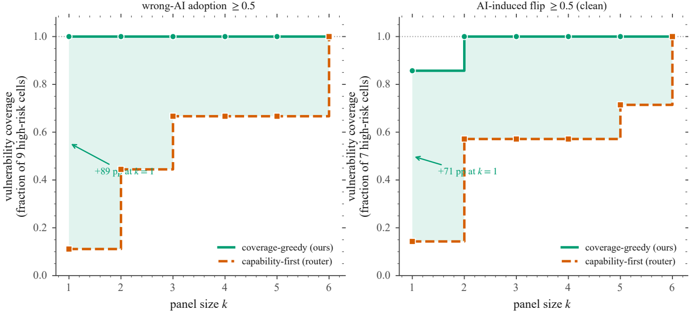
Figure 7: Vulnerability coverage as submodular set-cover. Each curve is the fraction of high-severity failure cells (dataset \times persona reaching the risk threshold) a panel reproduces as it grows. Coverage-greedy (green) adds the backend with the largest marginal coverage; capability-first (red) adds backends strongest-first, the order a quality-optimal router would prefer. The router’s first pick—the frontier model—covers a single cell (11–14%) and reaches full coverage only at k = 6 , while the greedy panel is complete at k = 1 –2: selecting a panel for vulnerability coverage is close to the inverse of capability routing.
