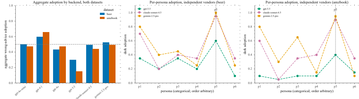
Fig. 4. Left: aggregate wrong-advice adoption spans a wide range across backends on both datasets. Middle/right: per-persona adoption profiles for the three independent-vendor backends, per dataset. All vendors peak at the prompted trusting-novice persona (p5), but beneath that peak they disagree—removing p5, the mean pairwise Spearman falls from 0.87 to 0.77 on beer and from 0.50 to 0.09 on amzbook. Persona order is categorical (arbitrary). The shared p5 peak is a property of the persona prompt, not population discovery.
