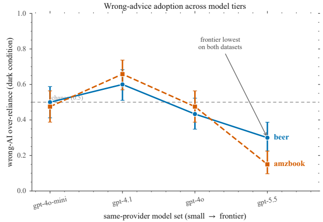
Figure 1: Axis-2 wrong-advice adoption on the guaranteed-wrong interface across the same-provider model set (gpt-4o-mini \rightarrow gpt-4.1 \rightarrow gpt-4o \rightarrow gpt-5.5), both datasets. Error bars are Wilson 95% binomial confidence intervals (descriptive; conflict-conditioned inference uses the item-clustered models below). Lines connect discrete model conditions only as a visual guide; the dashed line marks 0.5. Adoption is non-monotonic across backends; gpt-5.5 has the lowest adoption on both datasets. The matched framing contrast (Section 5.3) provides a non-arbitrary baseline for this low level.
