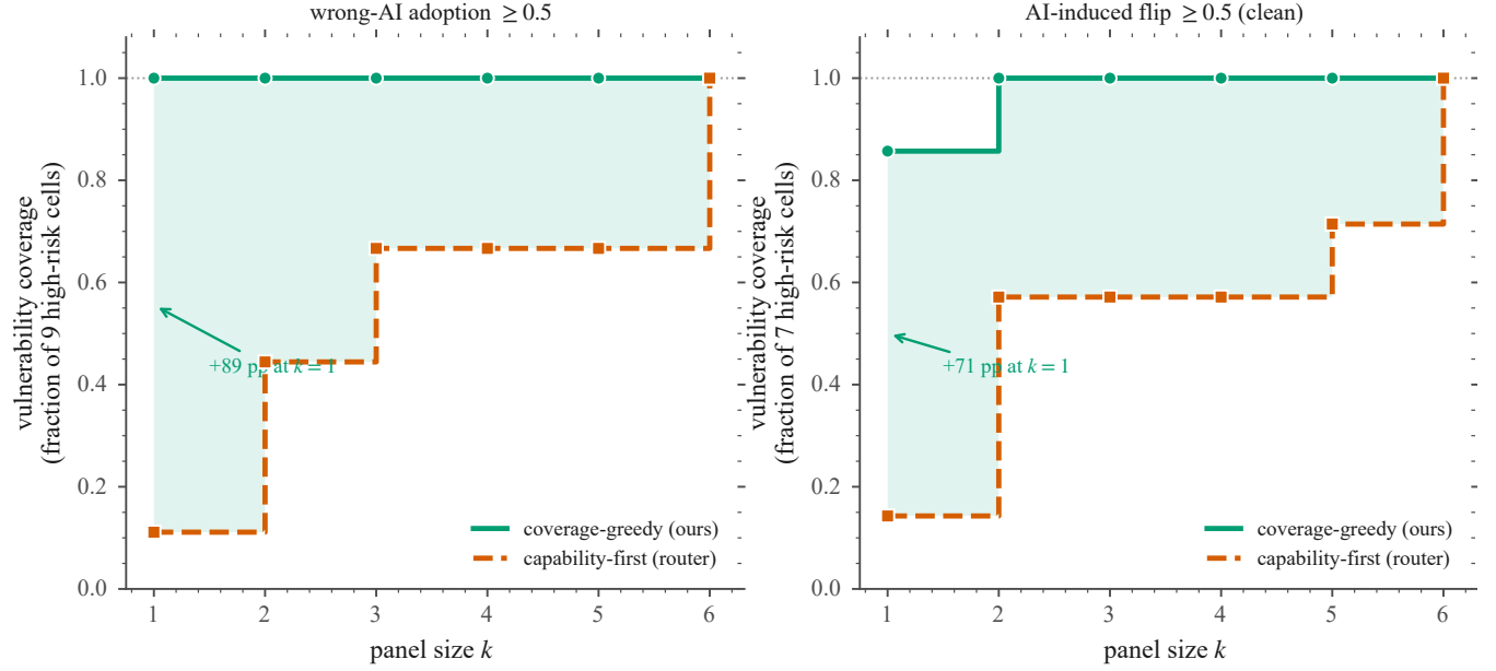
Figure 8: Vulnerability coverage as submodular set-cover. Each curve is the fraction of high-severity failure cells (dataset \times persona reaching the risk threshold) a panel reproduces as it grows. Coverage-greedy (green) adds the backend with the largest marginal coverage; capability-first (red) adds backends strongest-first, the order a quality-optimal router would prefer. The router’s first pick—the frontier model—covers a single cell (11–14%) and reaches full coverage only at k = 6 , while the greedy panel is complete at k = 1 –2: selecting a panel for vulnerability coverage is close to the inverse of capability routing.
