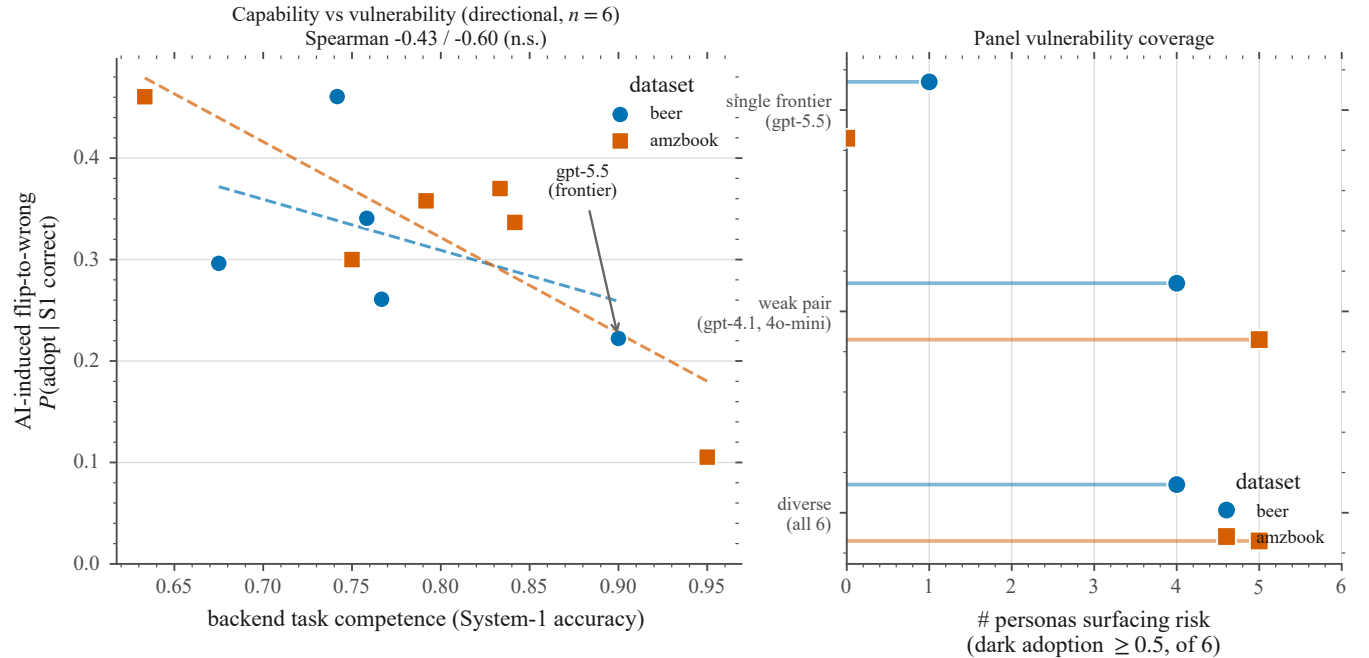
Figure 6: Left: backend task competence (System-1 accuracy) vs. the AI-induced flip rate P(\text{adopt} \mid \text{System-1 correct}) , both datasets—a directional negative trend (Spearman -0.43 / -0.60 ; n.s. at n=6 ). Right: vulnerability coverage (number of the six personas whose dark adoption reaches 0.5) for a single frontier backend, a weak pair, and the full panel. The single frontier backend surfaces the fewest at-risk profiles.
