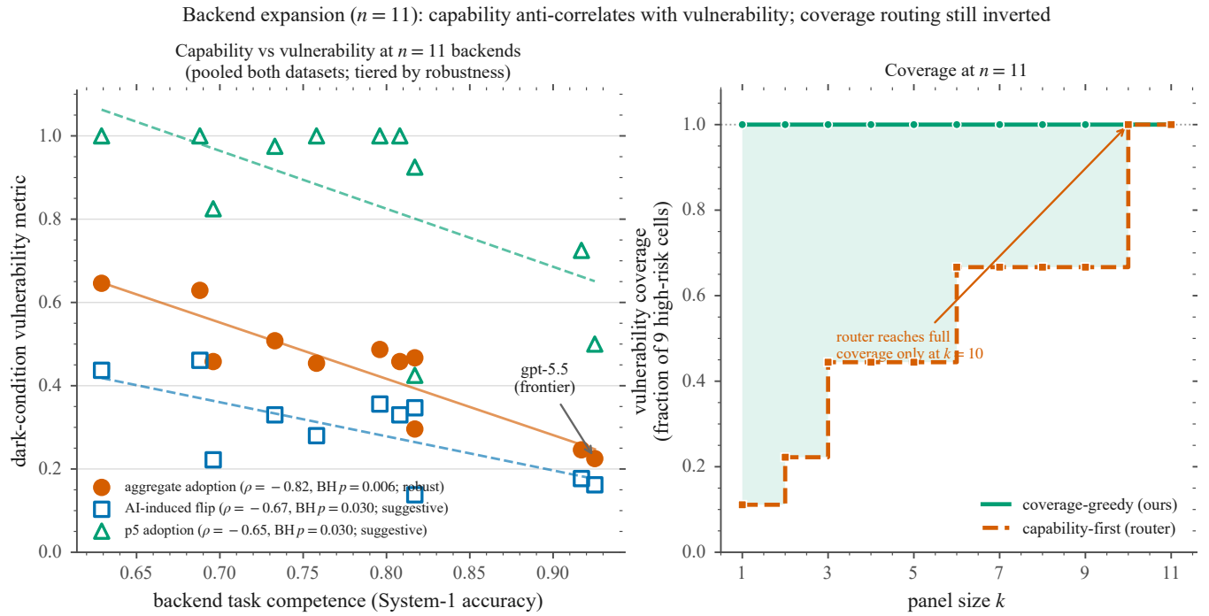
Figure 7: Backend expansion to n=11 (pooling both datasets). Left: backend task competence (System-1 accuracy) vs. three dark-condition vulnerability measures, tiered by robustness—aggregate adoption (filled, solid fit) is jackknife-robust and significant in each dataset; AI-induced flip and p5 adoption (open, dashed fit) are BH-significant only pooled and are amzbook-carried / single-backend fragile. Right: the n=11 vulnerability-coverage curve—a capability-first (router) panel reaches full coverage of the high-risk cells only at k=10 , while a coverage-greedy panel is complete almost immediately; a single frontier backend covers 1/9.
