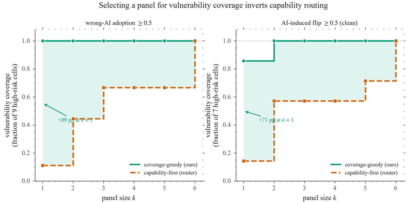
Figure 8: Vulnerability coverage as submodular set-cover. Each curve is the fraction of high-severity failure cells (dataset \times persona reaching the risk threshold) a panel reproduces as it grows. Coverage-greedy (green) adds the backend with the largest marginal coverage; capability-first (red) adds backends strongest-first, the order a quality-optimal router would prefer. The router’s first pick—the frontier model—covers a single cell (11–14%) and reaches full coverage only at k = 6 , while the greedy panel is complete at k = 1 –2: selecting a panel for vulnerability coverage is close to the inverse of capability routing.
