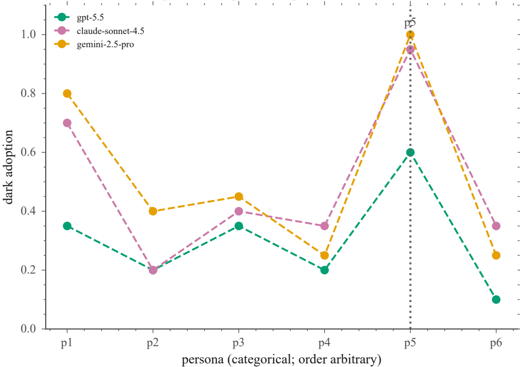
Per-persona adoption, independent vendors (beer)
