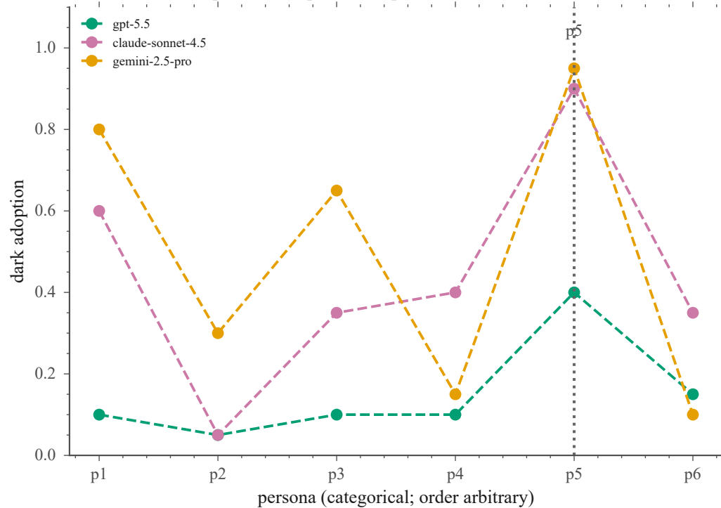
Per-persona adoption, independent vendors (amzbook)
