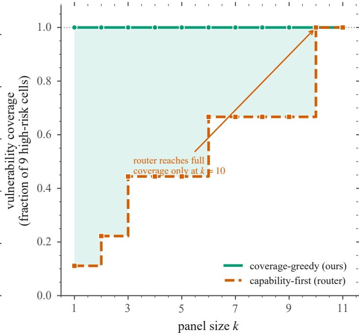
Coverage at n = 11
