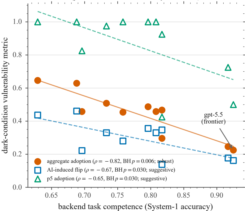
Capability vs vulnerability at n = 11 backends (pooled both datasets; tiered by robustness)
