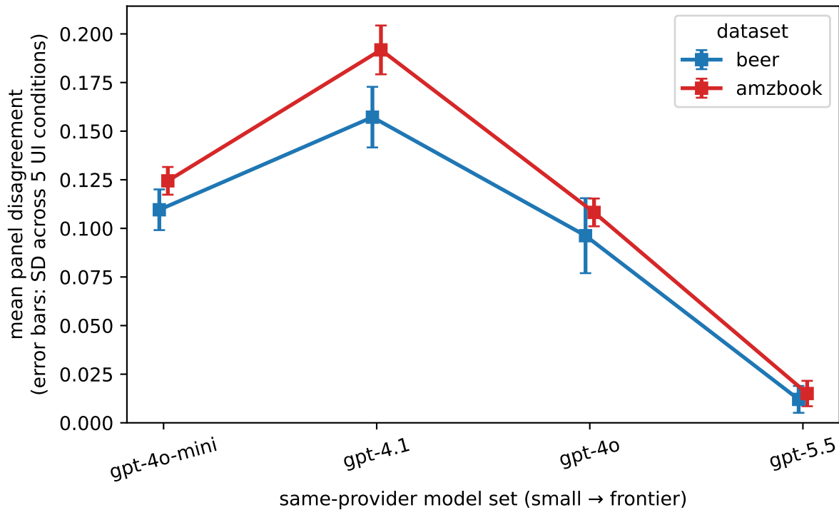
Mean panel disagreement by backend, both datasets
