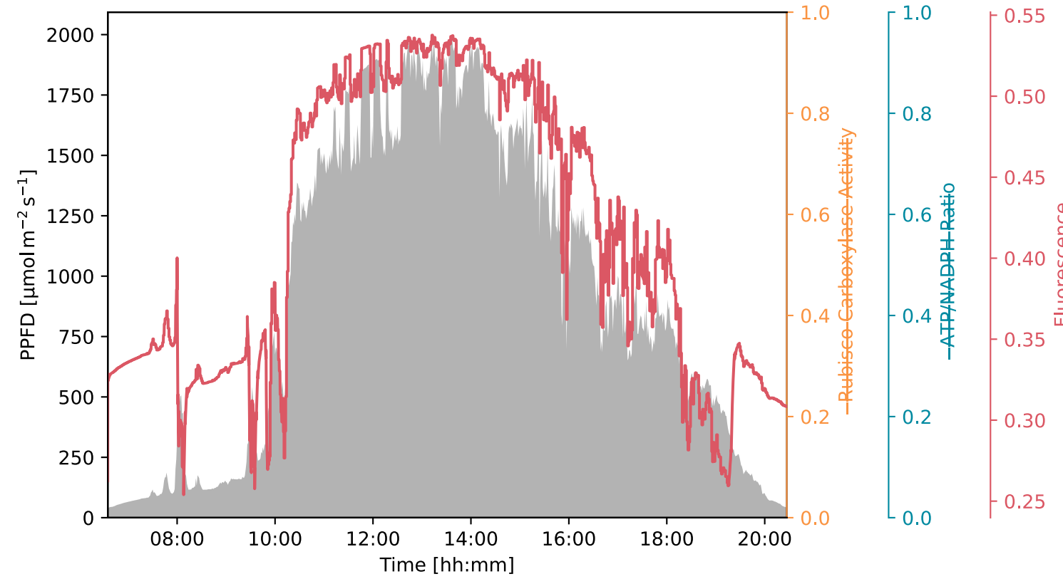
Matuszynska2016
