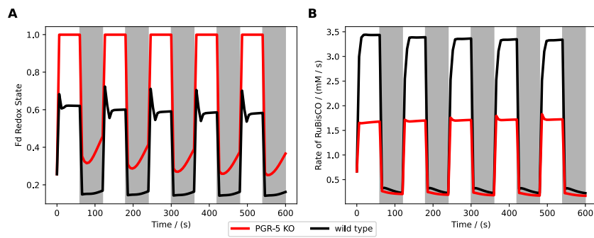
Figure 21: Comparison of results of a WT and knockout mutant simulation under varying light intensities.
