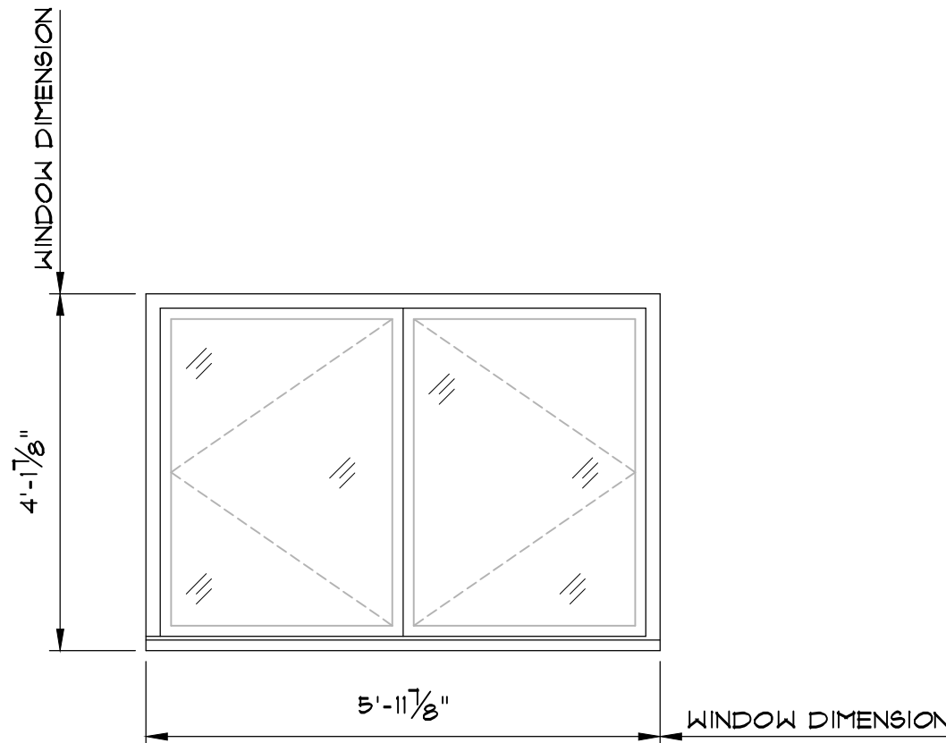
W-3 CASEMENT WINDOW
