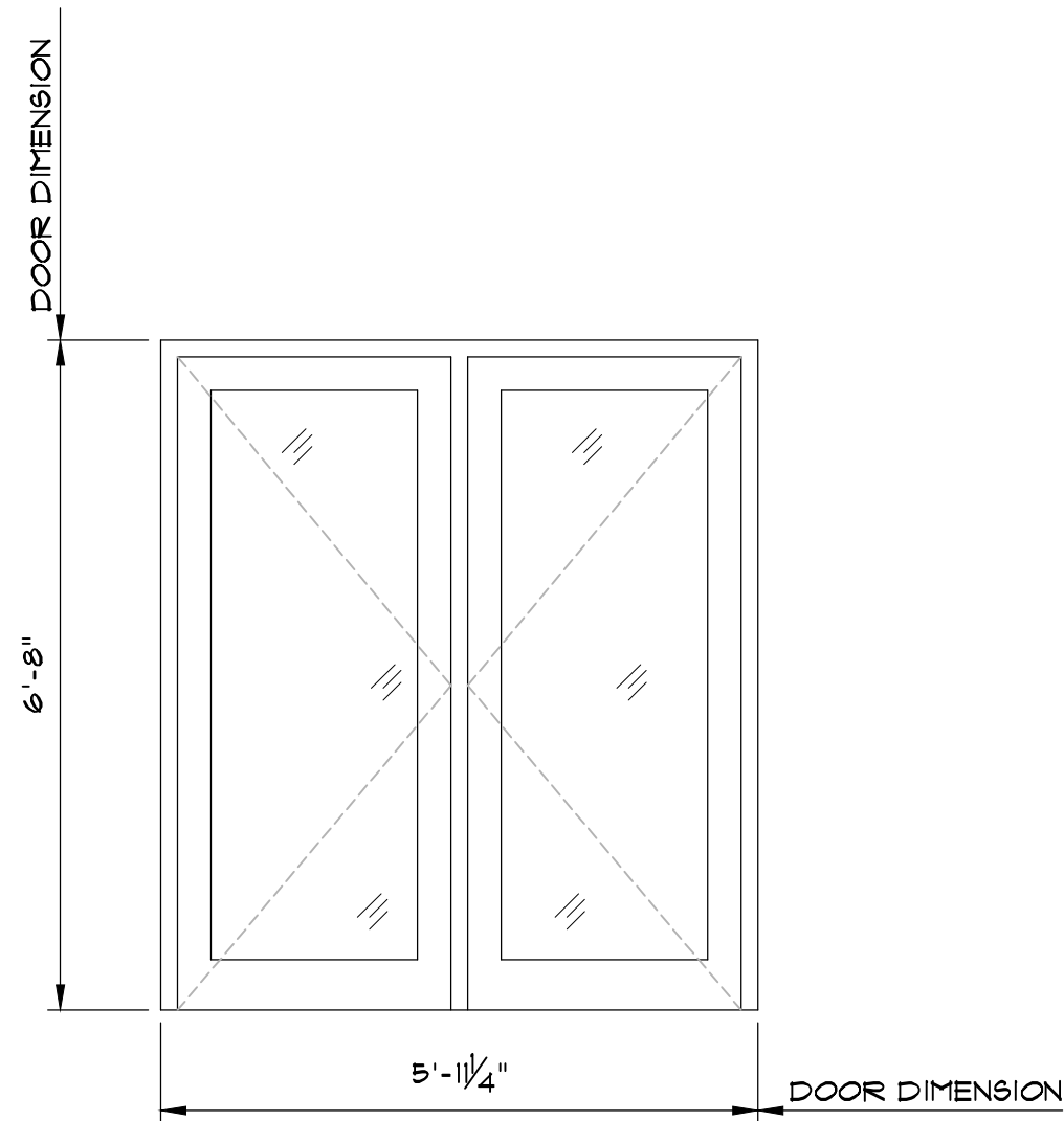
D-2 FRENCH HINGED PATIO DOOR - INSWING
