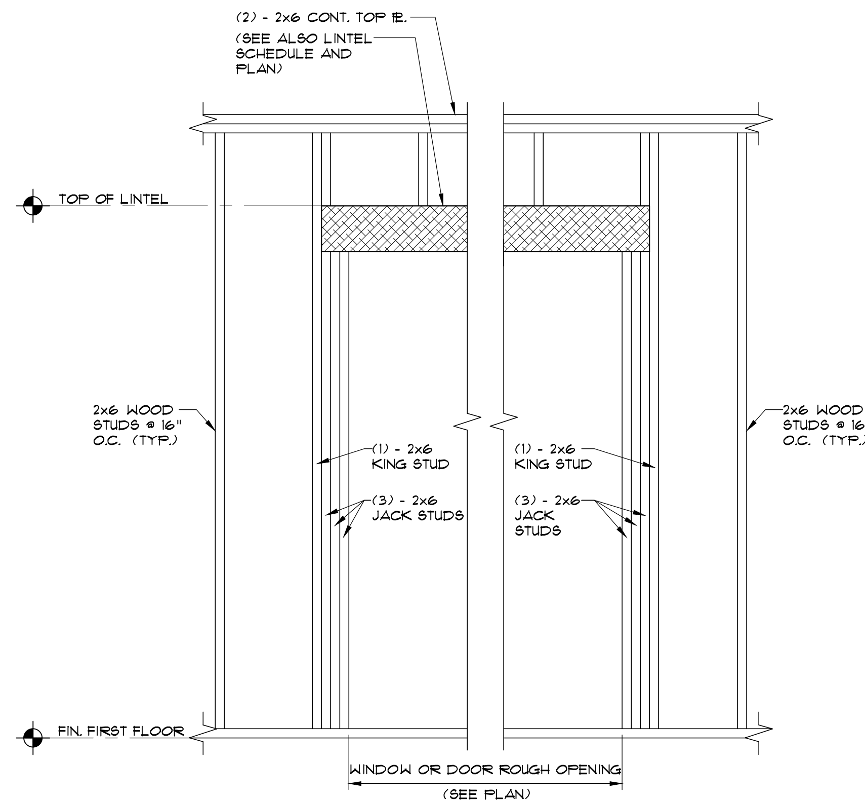
5 DETAIL: TYPICAL WINDOW / DOOR LINTEL SCALE: 3/4" = 1'-0"
