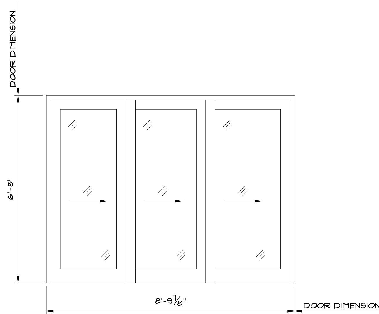
D-3 MULTI-SLIDE PATIO DOORS
