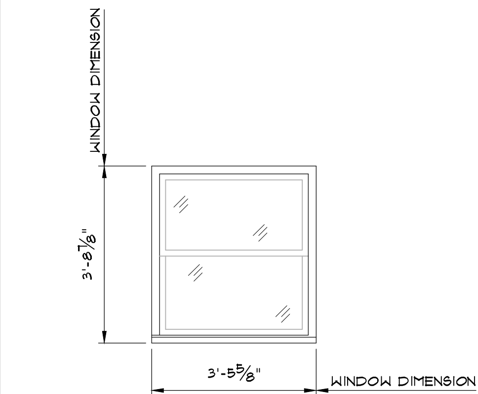
W-1 DOUBLE HUNG WINDOW
