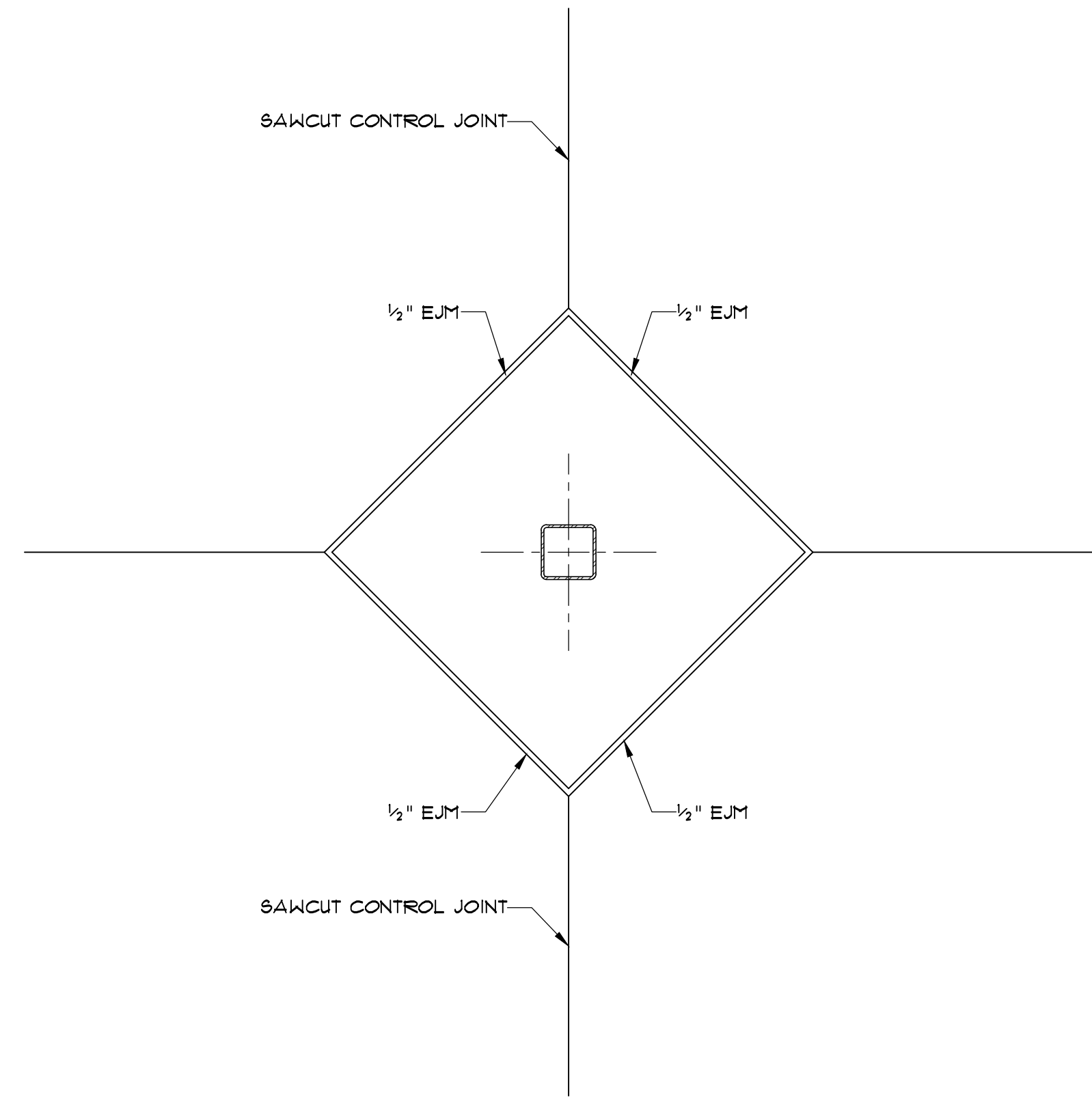
2 DETAIL: COLUMN ISOLATION CORNER SCALE: 1" = 1'-0"
