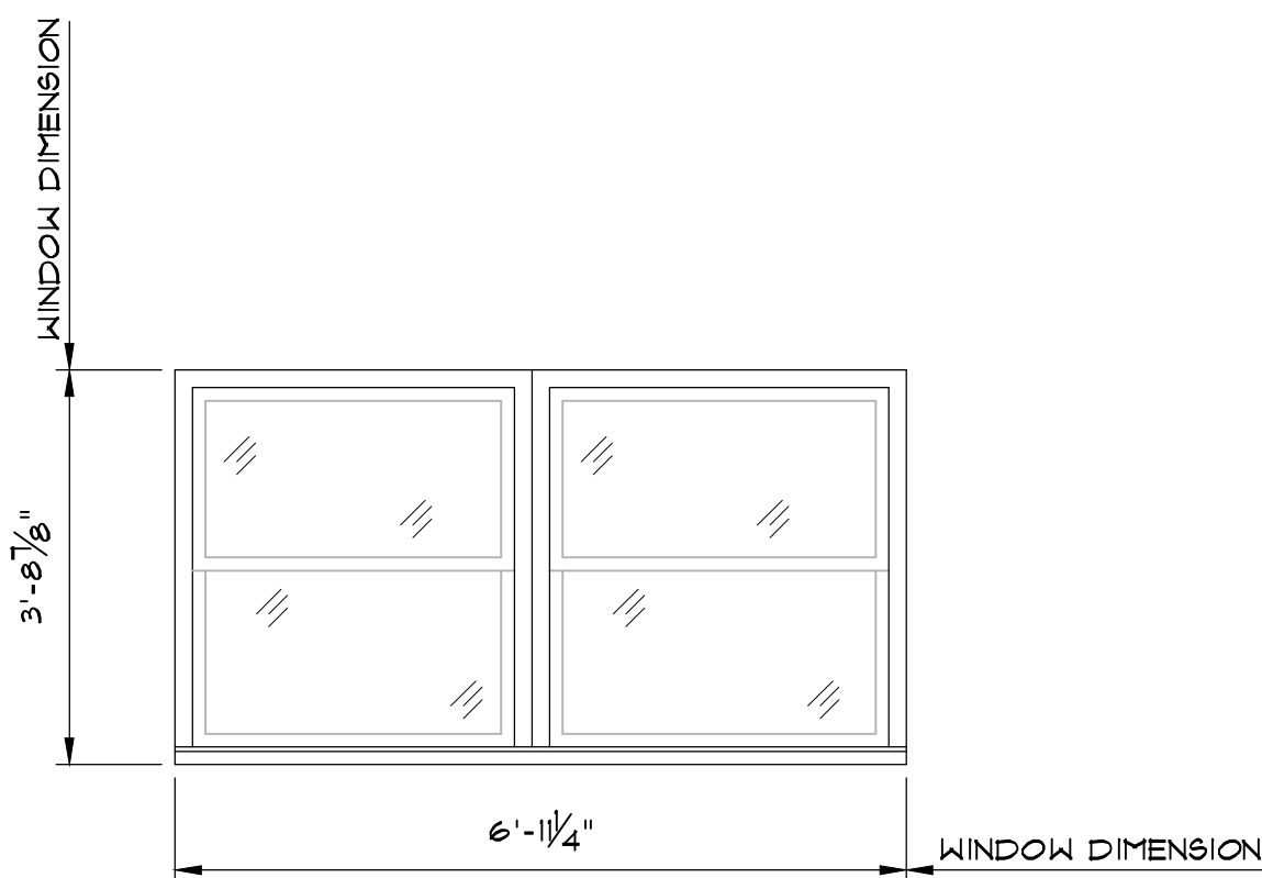
W-2 (TWO) DOUBLE HUNG WINDOW
