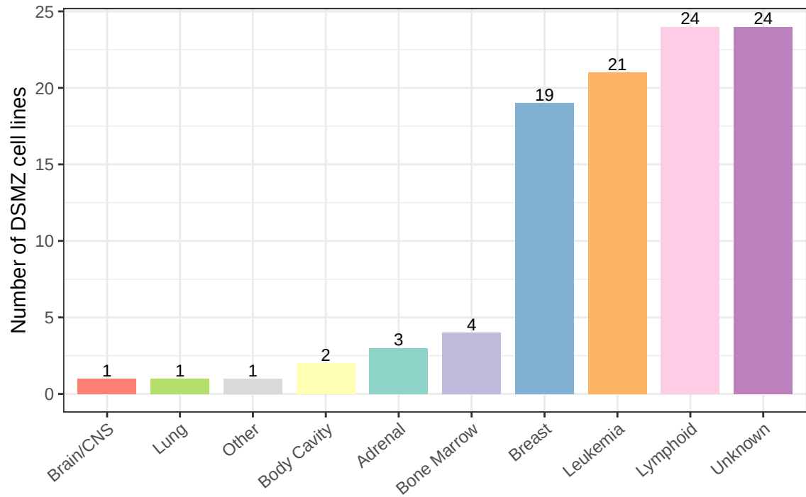
Organ distribution of DSMZ collection
