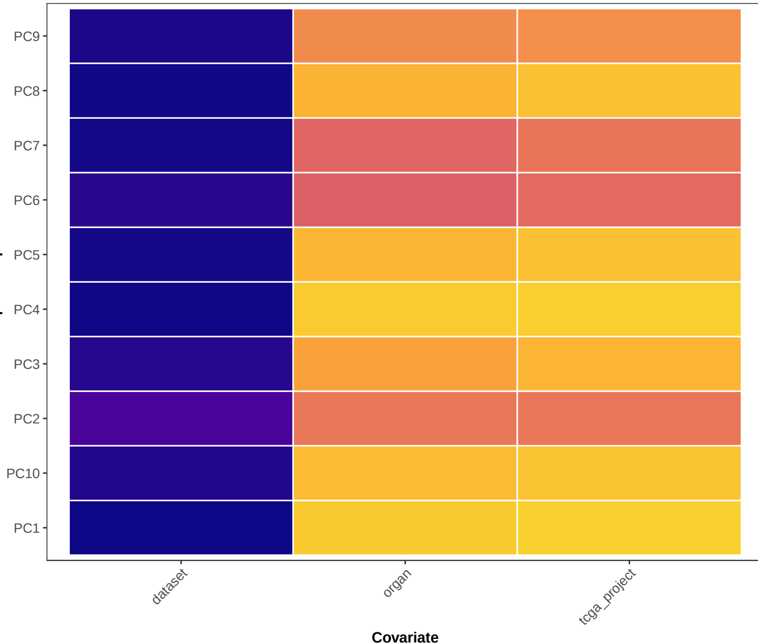
PC ... covariate R 2 (before)
