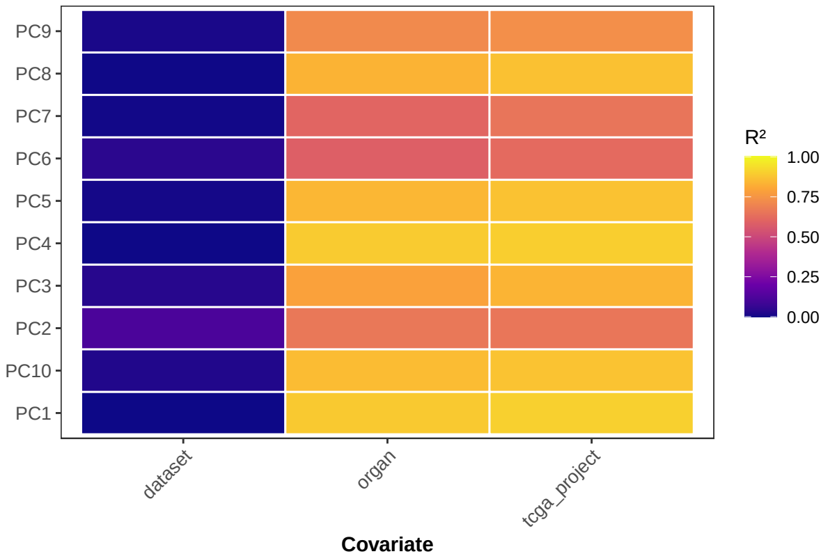
PC ... covariate R 2 (before)
