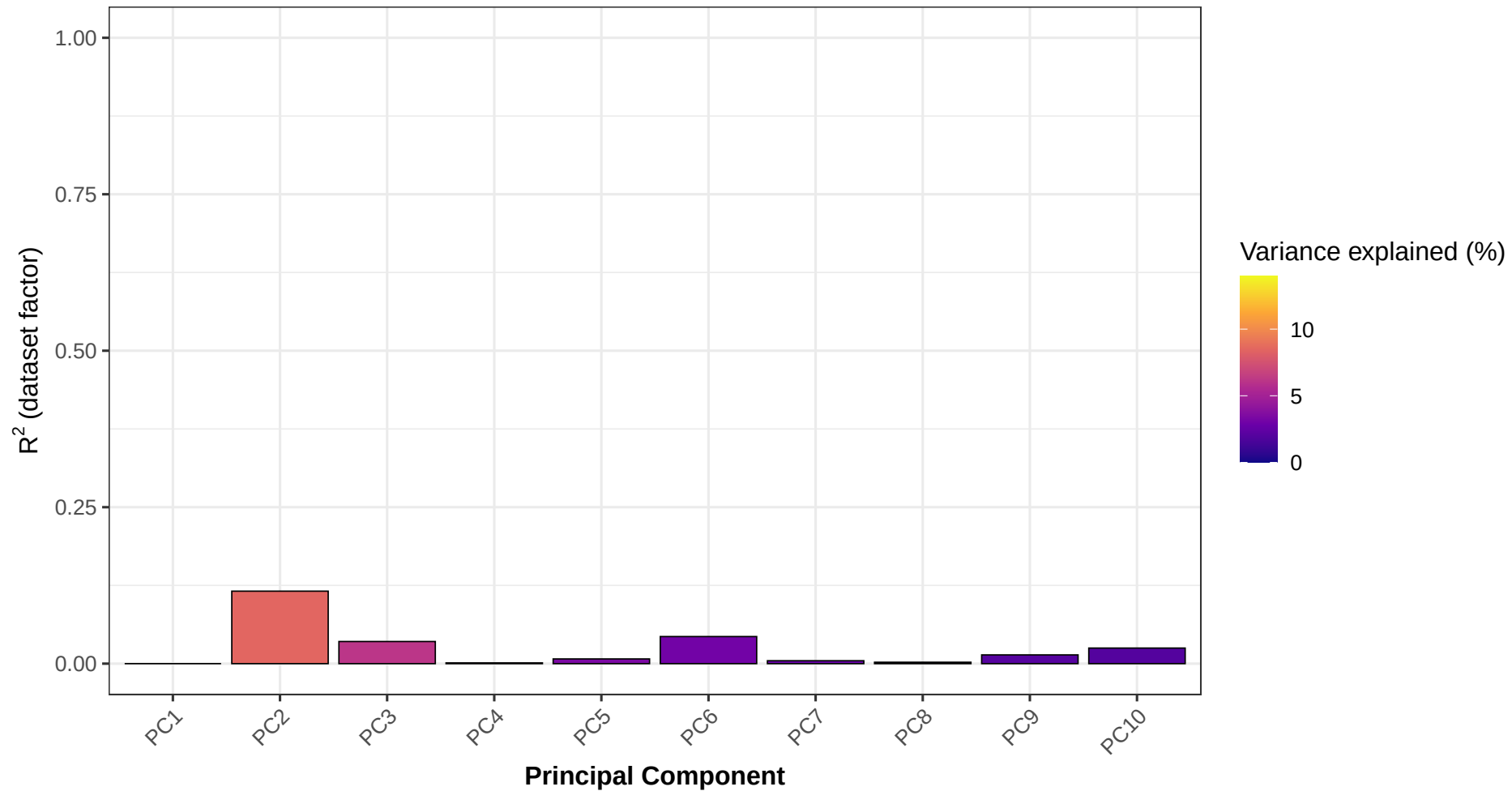
Top 10 PCs (48.4% cumulative variance)
