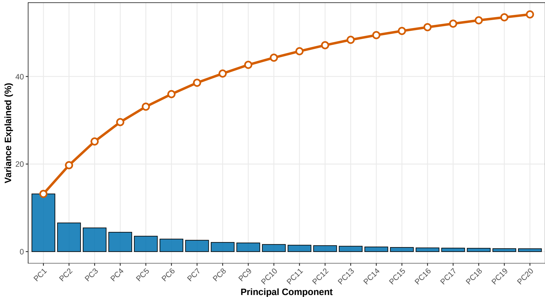
Scree Plot ... after
