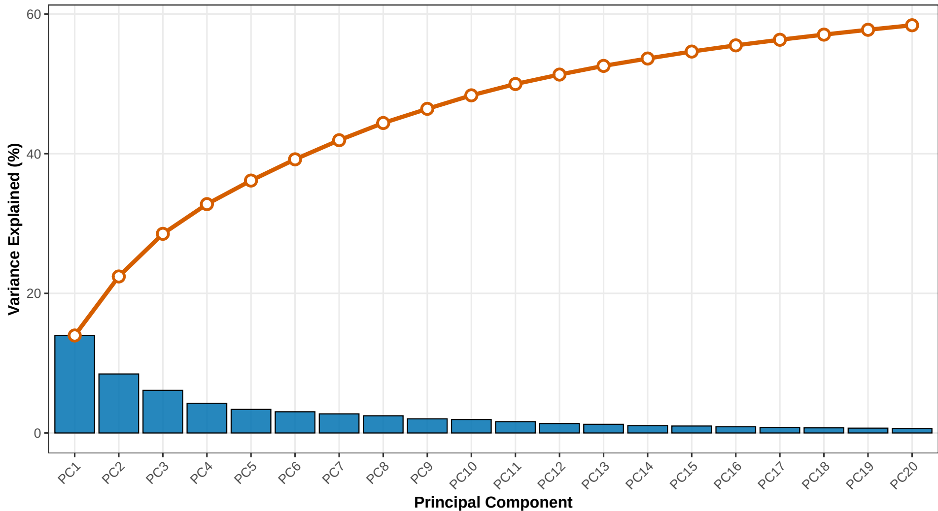
Scree Plot ... before
