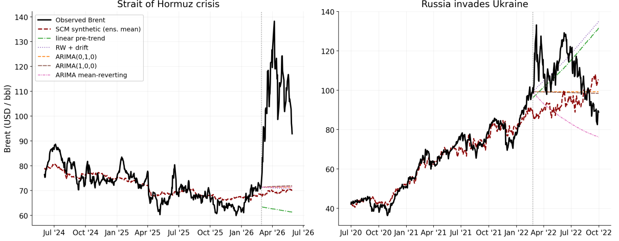
Figure 8: SCM vs. donor-free naive univariate counterfactuals.
