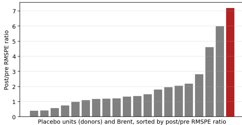
Figure 4: In-space placebo for Hormuz (convex SCM).
