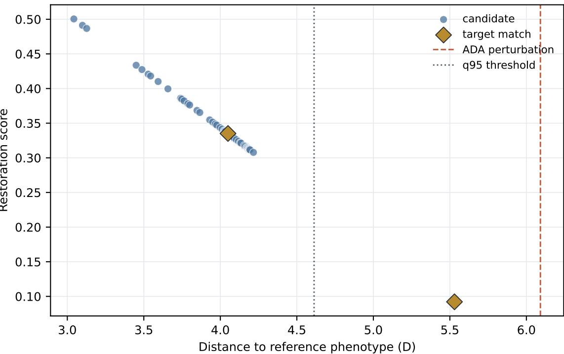
C. Distance-domain restoration benchmark, n=50
