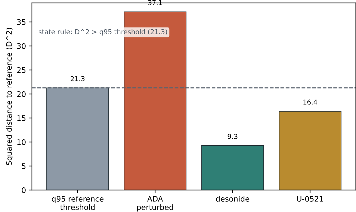
C. Distance-domain restoration benchmark, n=50
