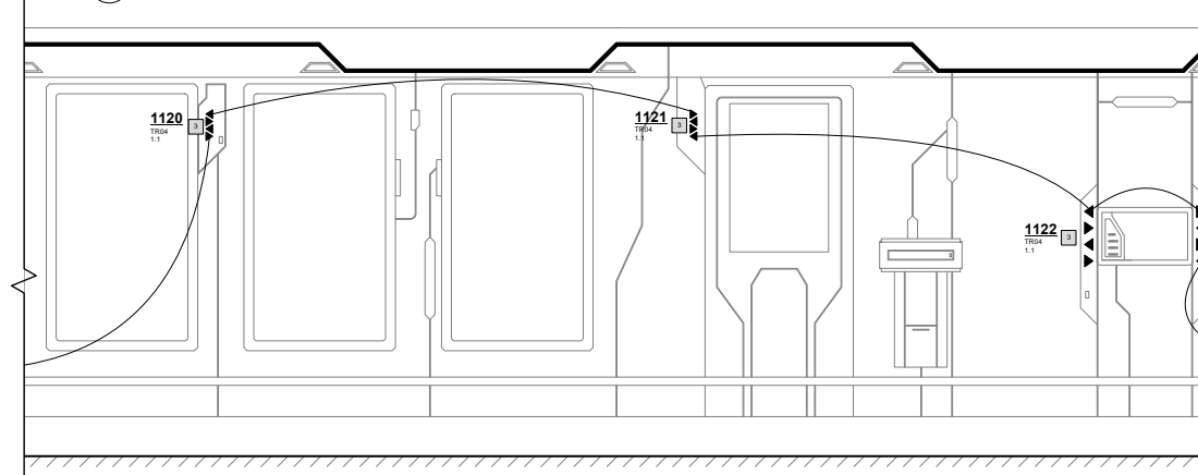
6 Space Elevator Developed Elevation 2 - 太空电梯立面展开图2 1:75
