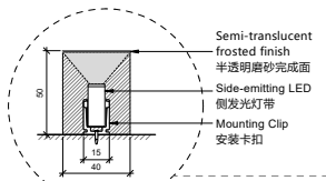
2 TR02 Hand Rail Underside LED Tape light Installation Detail 栏杆底部灯带安装示意图
