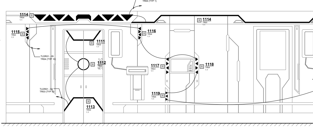
5 Space Elevator Developed Elevation 1 - 太空电梯立面展开图1 1:50
