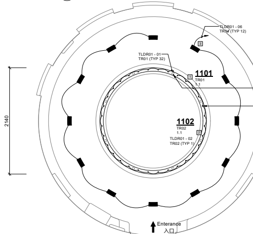
4 Space Elevator plan view (ground) - 太空电梯平面图(地面) 1:75
