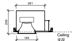
4 TR05 RGBW recessed ceiling downlight Ø152.4 mm cut-out RGBW 天花筒灯, 开孔尺寸Ø152.4 mm
