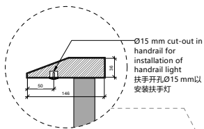
1 TR01 Hand Rail Light Installation Detail 扶手灯安装示意图
