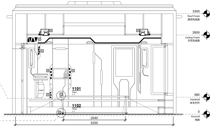
3 TR03, TR04 Illuminated surface decoration (By others) 装饰发光面(其他供应商)
