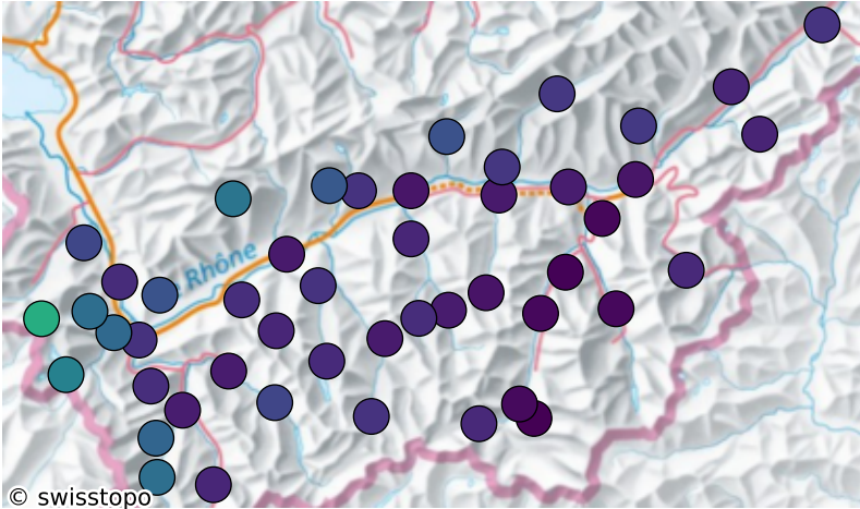
LSTM
