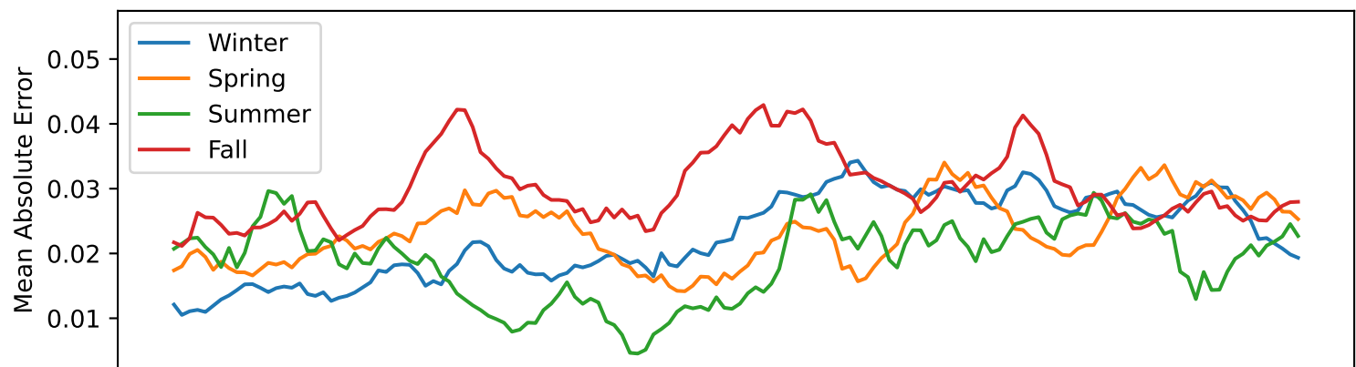
Architecture: LSTM
