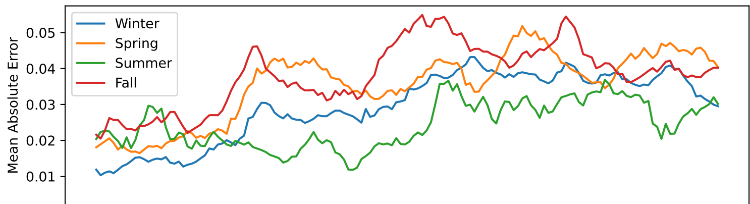
Architecture: KAN
