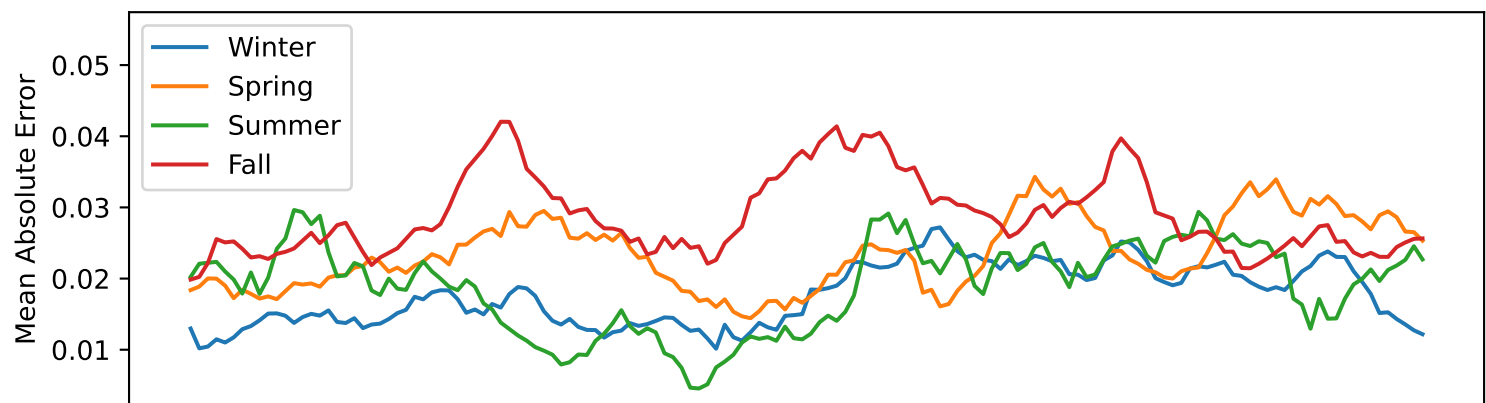
Architecture: MLP
