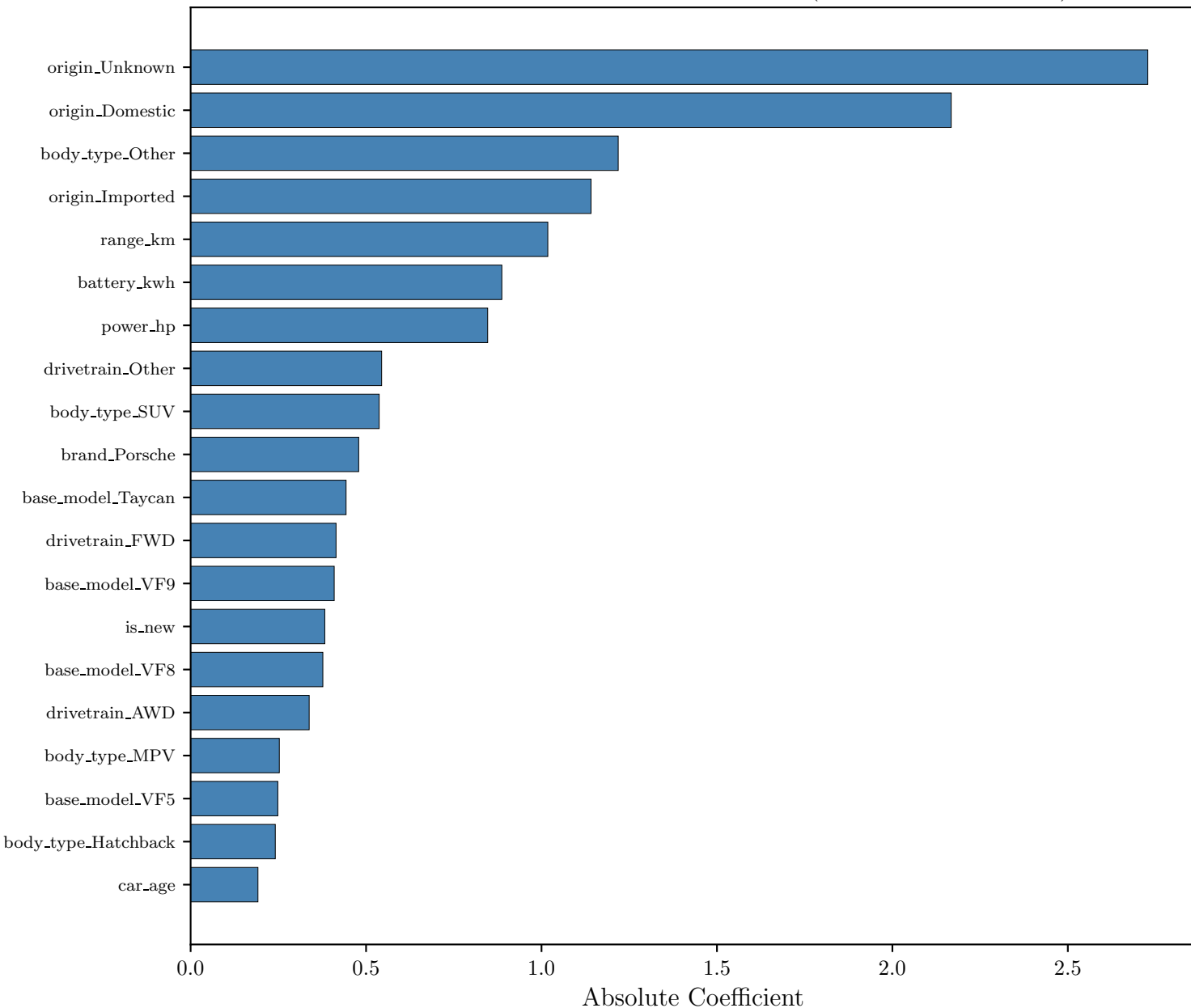
Linear Regression — Top 20 Features (Absolute Coefficient)
