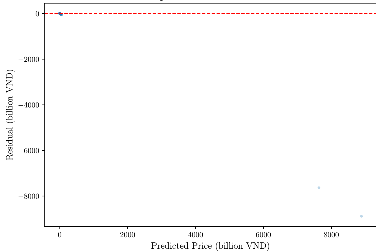
Linear Regression — Residuals vs Predicted
