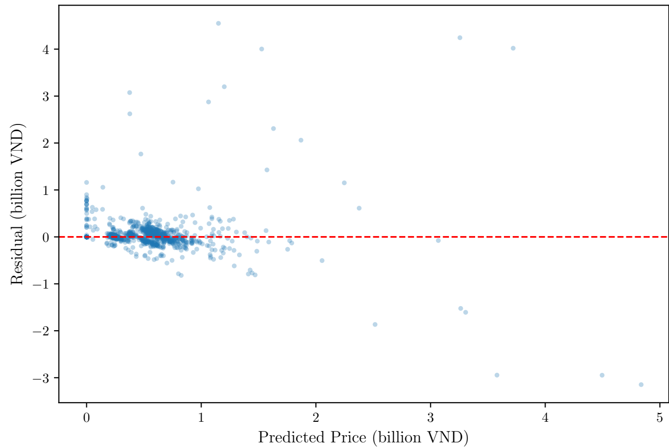
Svr — Residuals vs Predicted
