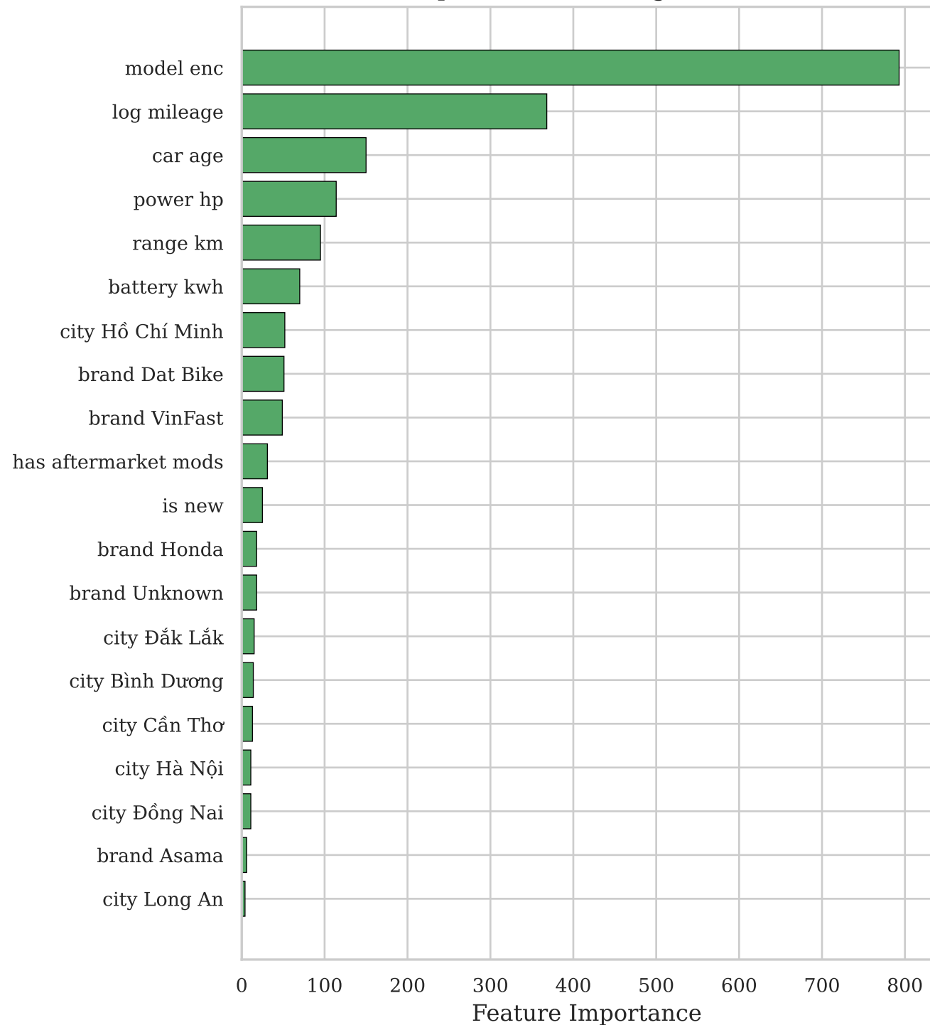
Top 20 Features (LightGBM)
