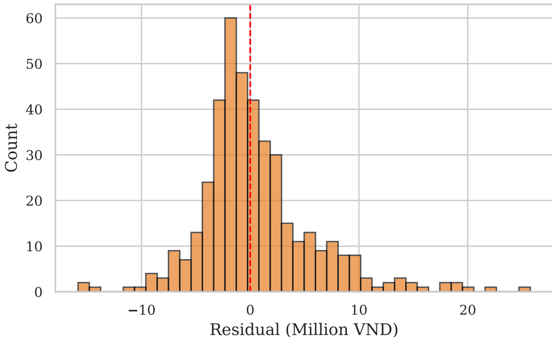
Residual Distribution (XGBoost)
