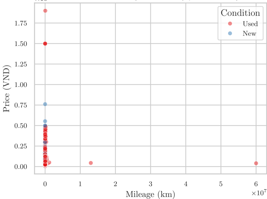
Interaction: Mileage vs Price (by Condition)
