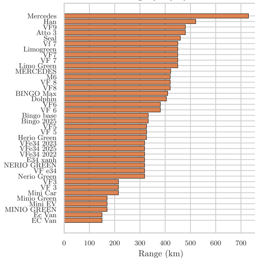
EV Range (km) by Model
