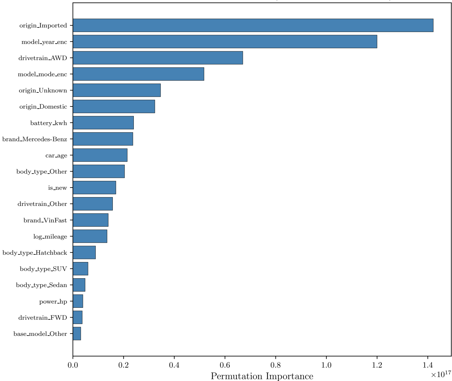
Lightgbm — Top 20 Features (Permutation Importance)
