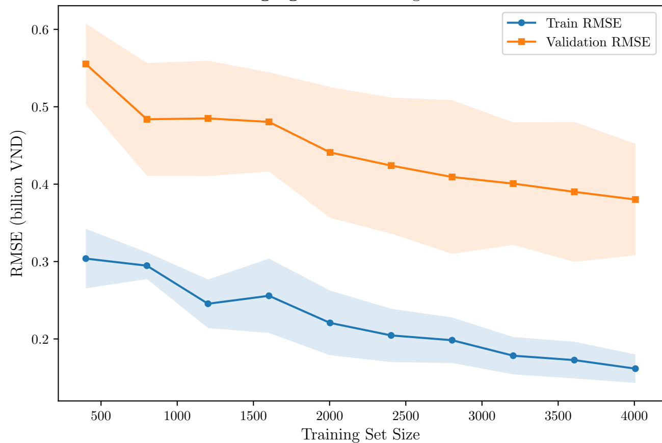
Lightgbm — Learning Curves
