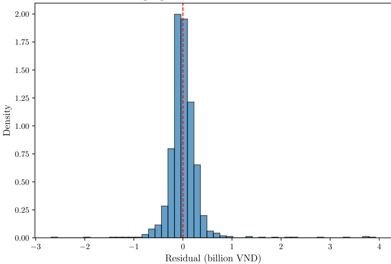
Lightgbm — Residual Distribution
