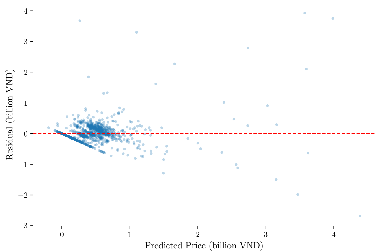
Lightgbm — Residuals vs Predicted
